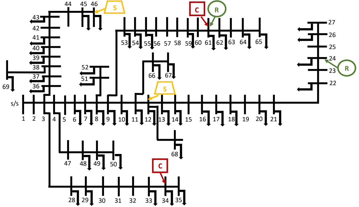
Figure 3.2: 69-bus system
