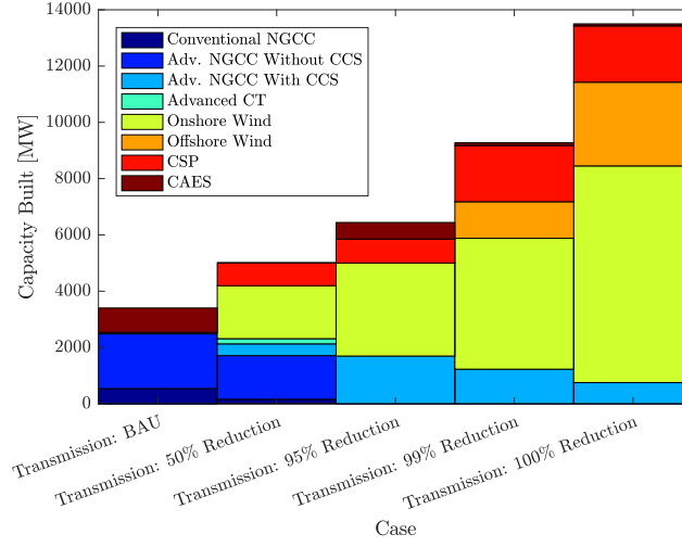
Figure 2.6: Capacity Built In Business-As-Usual Case and with Different Carbon-Emissions Reductions Relative to Business-As-Usual Case Under Transmission-Congestion Sensitivity Analysis
