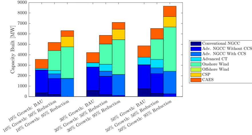
Figure 2.10: Capacity built in business-as-usual case and with different carbon-emissions reductions relative to business-as-usual case under electricity-demand sensitivity analysis.
