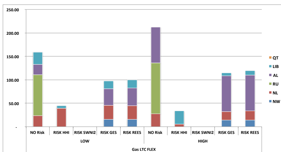
Figure 5.10: Volumes of natural gas exchanged via LTCs under the “Risk” and “FLEX” assumptions (mcm/day)
