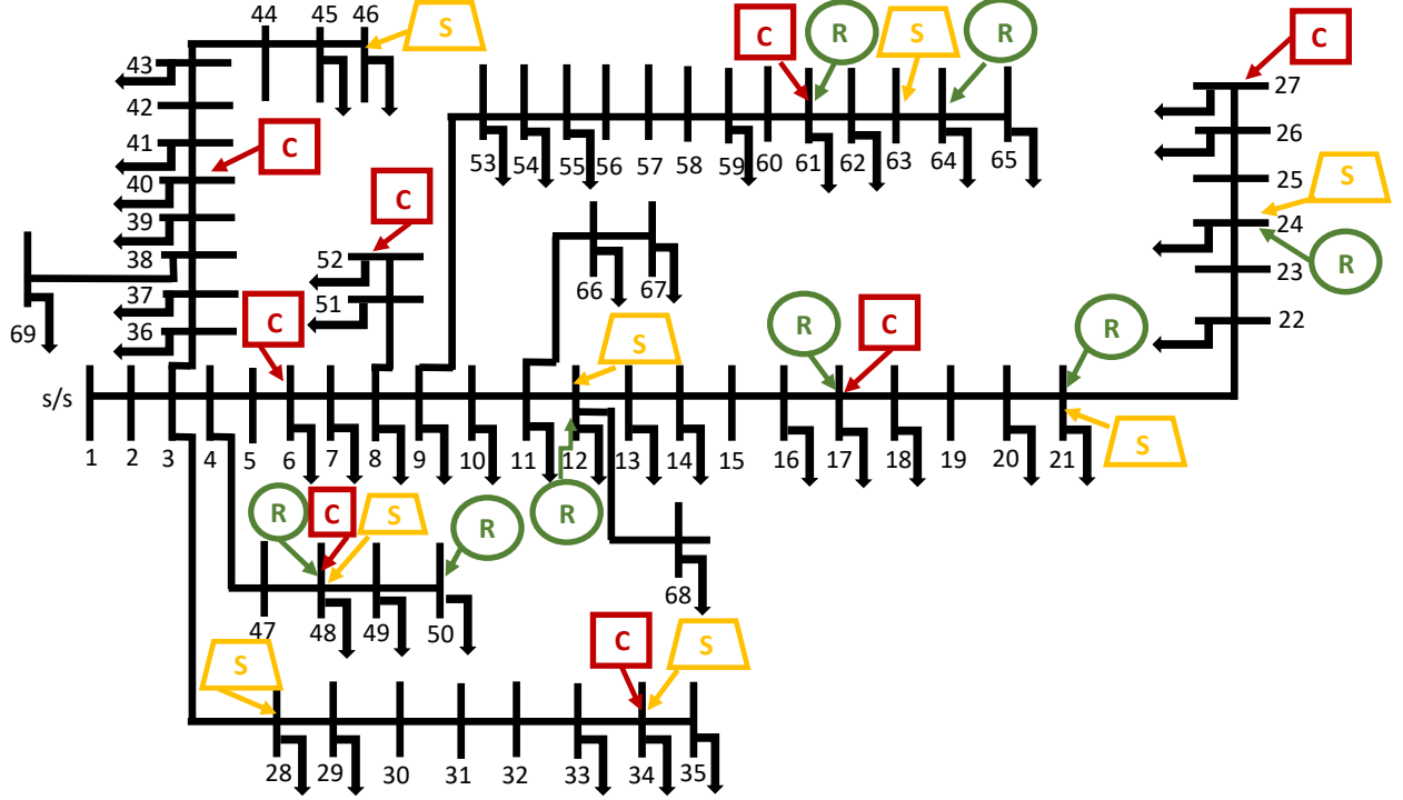
Figure 3.4: 69-bus system under the “8CN” the network configuration assumption
