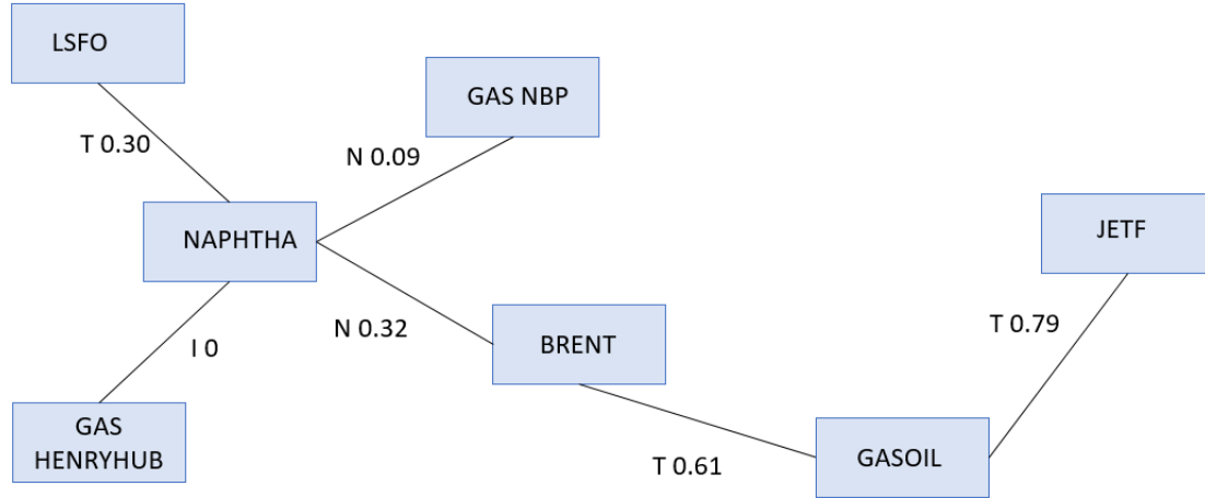
Figure 4.7: First tree of the R -vine with a 5% confidence level. The letters reported between the root nodes indicate the type of the bivariate copulas used to model the dependence, while the numbers refer to the corresponding Kendall's \tau correlation.
