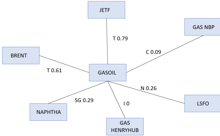
Figure 4.5: First tree of the C -vine with a 5% confidence level. The letters reported between the root nodes indicate the type of the bivariate copulas used to model the dependence, while the numbers refer to the corresponding Kendall's \tau correlation.
