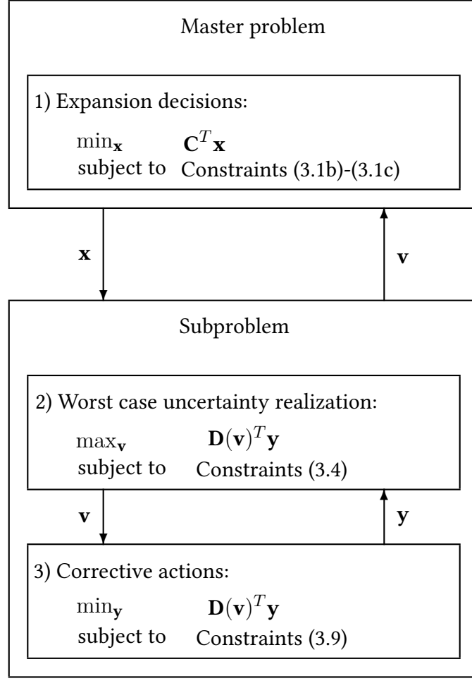
Figure 3.1: Iterative solution approach of the ARO problem
