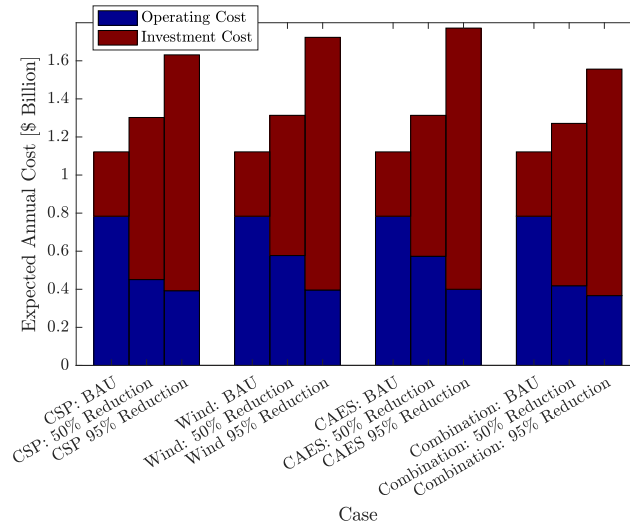
Figure 2.5: Expected Annual Operating and Investment Costs In Business-As-Usual Case and With Different Carbon-Emissions Reductions Relative to Business-As-Usual Case Under Technology-Improvement Sensitivity Analysis
