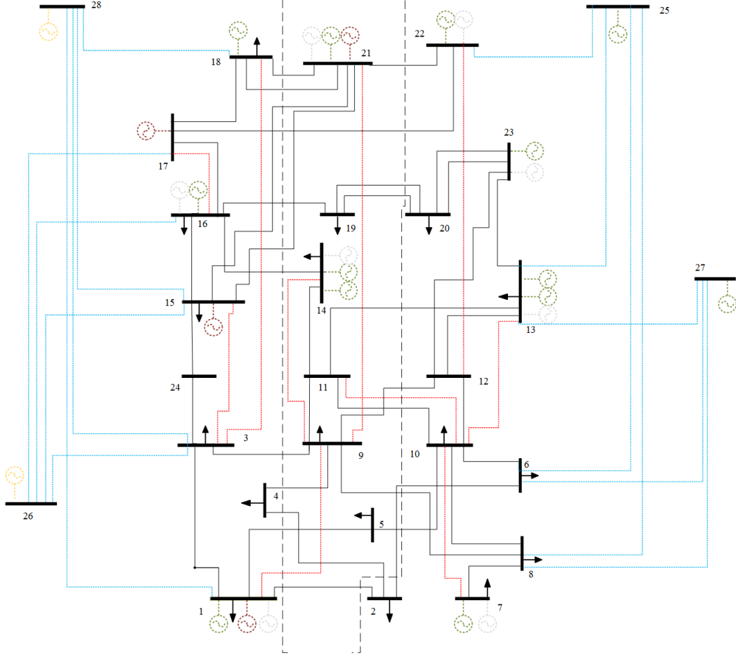
Figure 2.1: 28-Node Network Diagram
