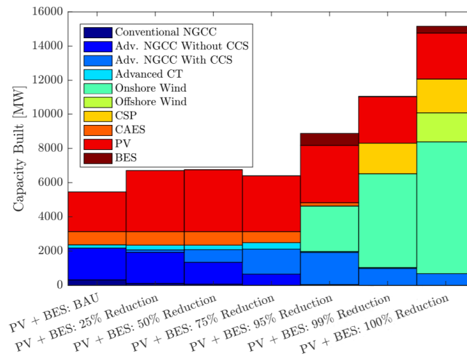
Figure 2.8: Capacity built in business-as-usual case and with different carbon-emissions reductions relative to business-as-usual case under PV-solar-and-BES sensitivity analysis
