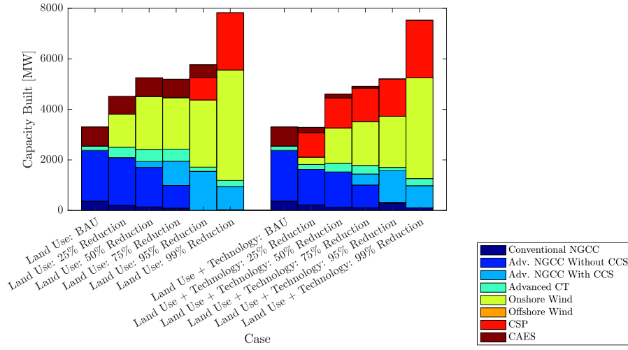
Figure 2.7: Capacity Built In Business-As-Usual Case and with Different Carbon-Emissions Reductions Relative to Business-As-Usual Case Under Land-Use Sensitivity Analysis
