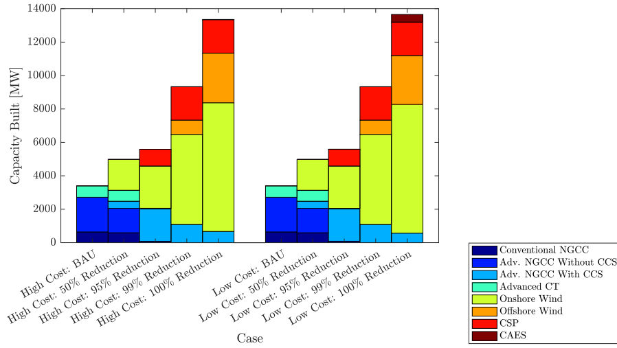
Figure 2.9: Capacity Built In Business-As-Usual Case and with Different Carbon-Emissions Reductions Relative to Business-As-Usual Case Under Adiabatic-CAES Sensitivity Analysis
