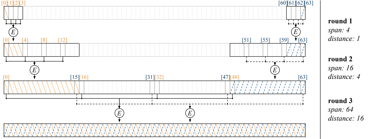
Figure 30: Propagation of the content of mini-blocks [0] and [63] in the mix process
