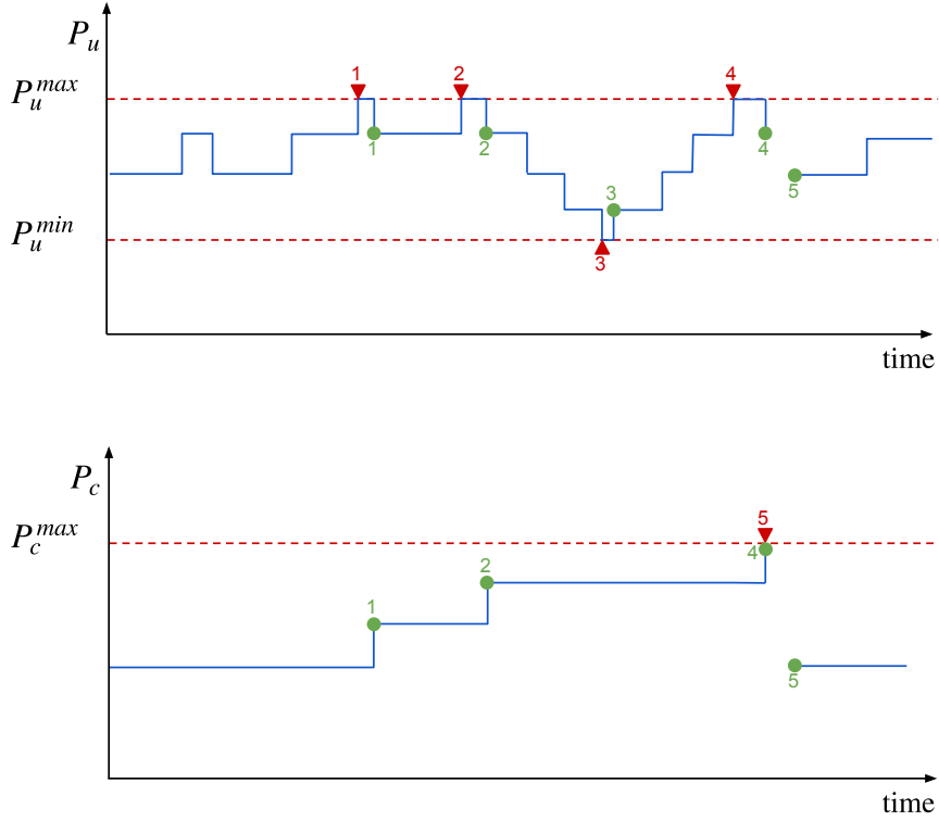
Figure 39: An example of evolution of P_u (top chart) and P_c (bottom chart) as a consequence of nodes leaving and re-joining the DCS and of actions taken by the data owner
