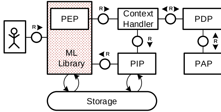
Figure 42: The proposed system architecture (including “ML Library” and “Storage” components integrated with those of OASIS XACMLv3 standard)
