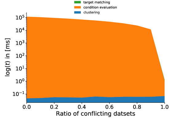
Figure 60: Total decision time for a complex policy
