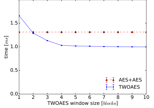
Figure 22: BEL+SEL encryption performance on a 1MB file using two subsequent AES invocations and TWOAES
