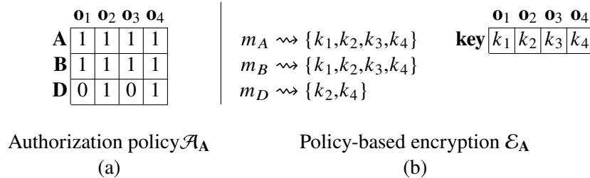
Figure 7: An example of authorization policy defined by user Alice (a) and corresponding policy-based encryption (b)
