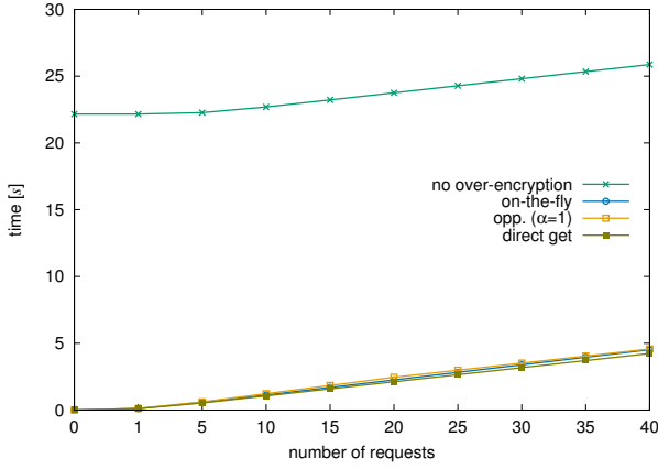
Figure 19: Overhead of all the solutions
