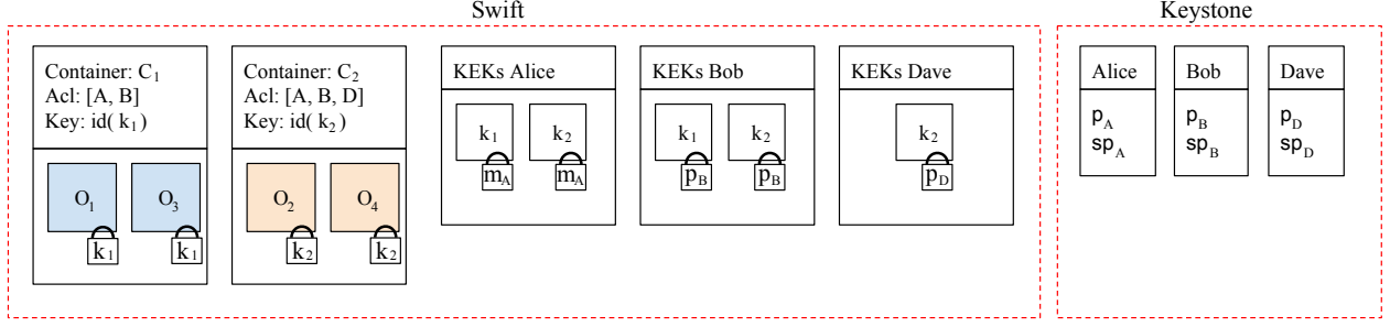
Figure 8: Policy-based encryption \mathcal{E}_A equivalent to the authorization policy \mathcal{A}_A in Figure 7(a)
