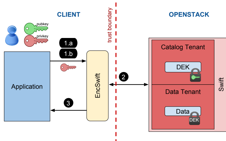
Figure 13: App-aware architecture
