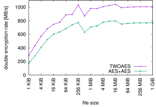
Figure 25: Re-encryption using AES-NI
