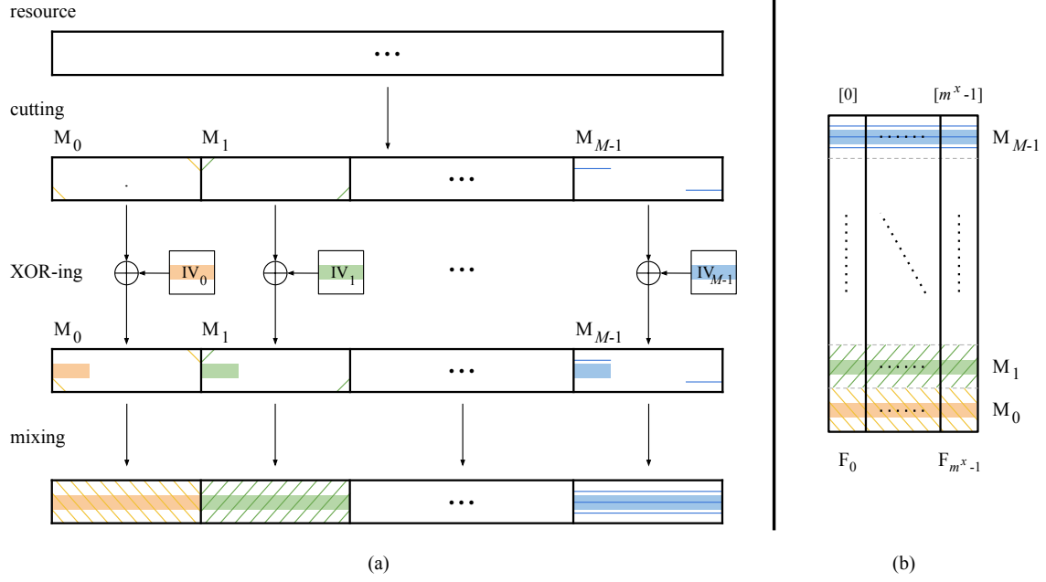
Figure 31: From resource to fragments
