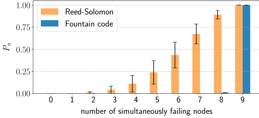
Figure 38: Probability that a resource becomes unavailable using Reed-Solomon and fountain codes, assuming p_u=0.015 , P_u^{min}=10^{-12} , P_u^{max}=10^{-5} , f=7 fragments, and s in [10,15]
