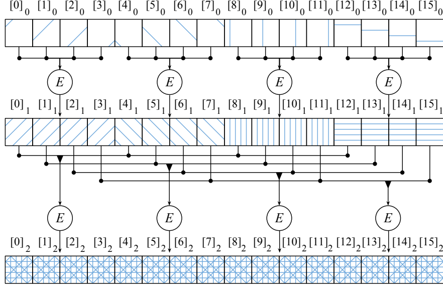
Figure 28: An example of mixing of 16 mini-blocks assuming m = 4
