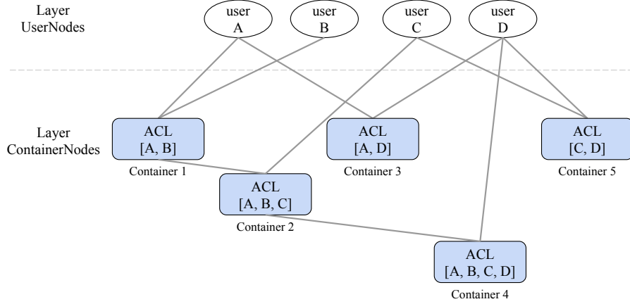
Figure 12: Graph with DEK derivation from other DEKs
