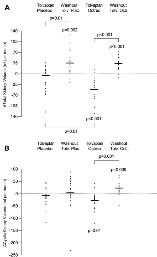
Figure 2. Changes in kidney volumes during the different study periods. Changes in total kidney volumes (A) and cystic kidney volume (B) during the two 1-month treatment periods with tolvaptan and placebo or with tolvaptan and octreotide-LAR add-on therapy as compared with changes during the two corresponding washout periods from tolvaptan and placebo and from tolvaptan and octreotide-LAR. The black points indicate values of each single individual during each study period and the horizontal bars show the mean of corresponding individual points. The P values without brackets indicate that changes observed in the considered variables in the considered period were significant. The P values with brackets show that the changes in the two considered treatment periods were significantly different.
