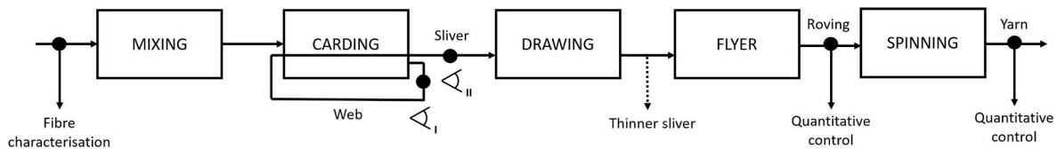
Fig. 12. Control points along the innovative spinning process.
