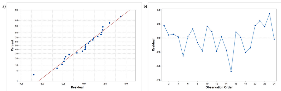
Fig. 17. a) Residual normal distribution and b) Randomly scattered residual.
