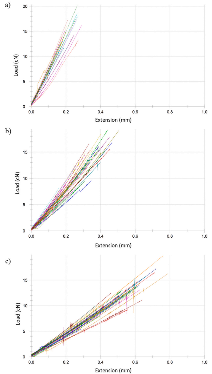
Fig. 3. Load-extension curves for 10 (a), 20 (b) and 40 (c) mm gauge length.
