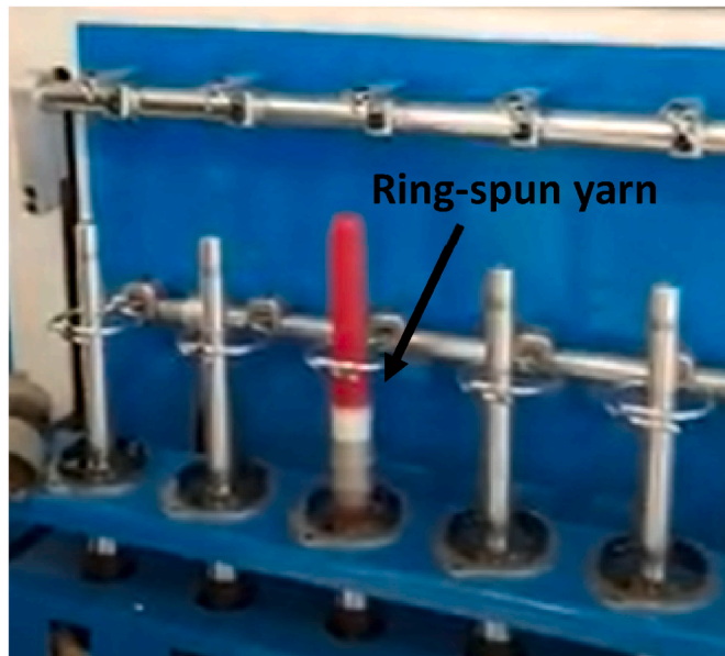
Fig. 11. Ring spinning machine adopted in the study with ring bobbin production.
