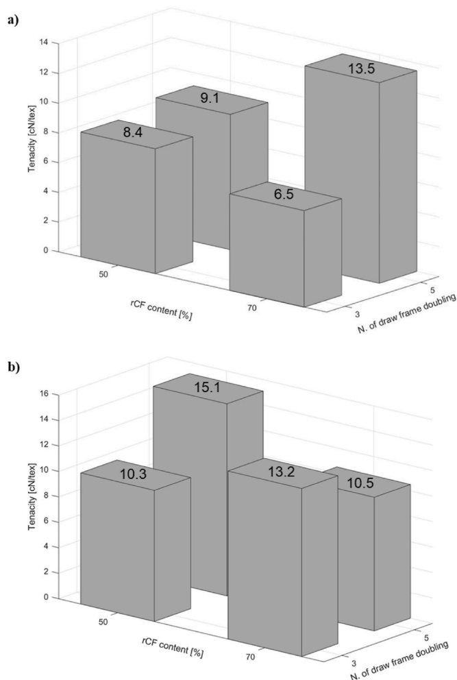
Fig. 15. Tenacity of ring-spun hybrid yarns considering rCF content and number of draw frame doubling for a) polyamide and b) polyester fibres.
