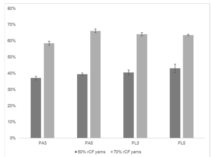
Fig. 16. Share of actual amount of recycled CF for all the hybrid yarns produced measured by TGA (standard deviations are shown as error bars).
