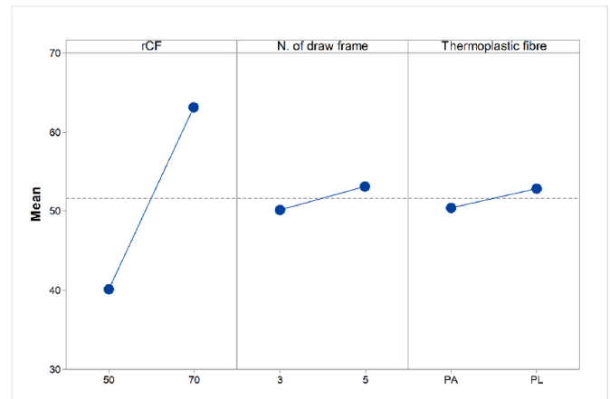
Fig. 18. Main effects plot for output.
