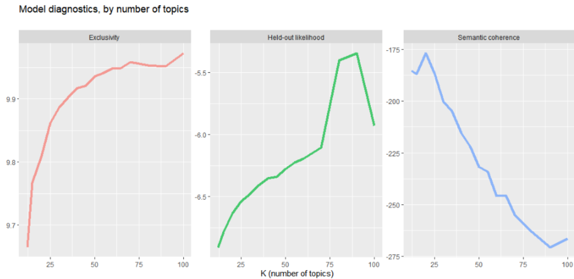
Figure 9 - STM diagnostics: held-out likelihood, semantic coherence, exclusivity, by K
