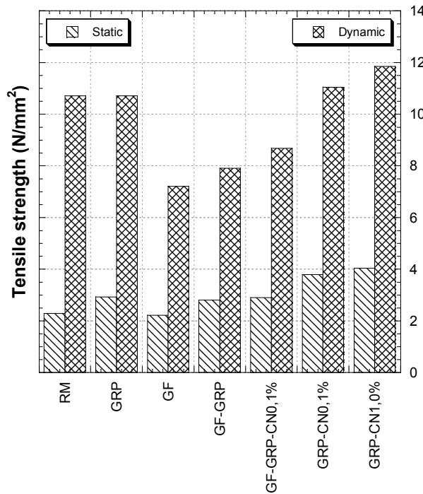
Figure 4 – Tensile strength on static and dynamic condition.
