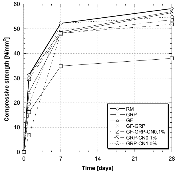
Figure 3 – Compressive strength vs. Time.
