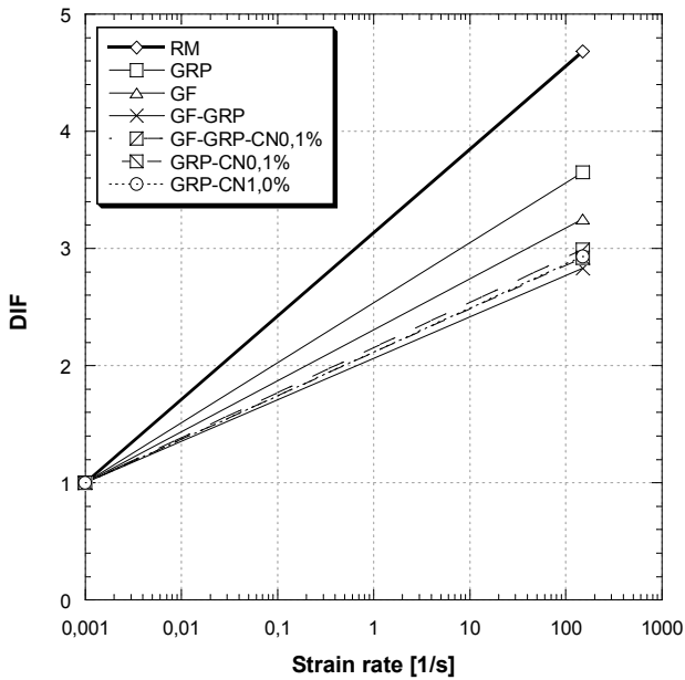
Figure 5 – Dynamic Increase Factor (DIF)
