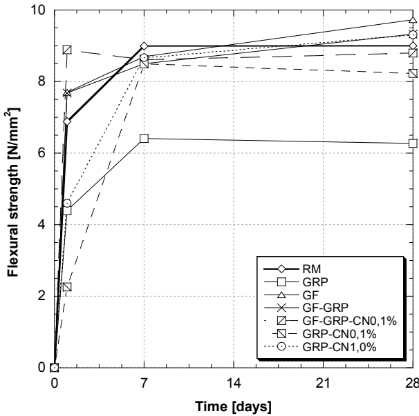
Figure 2 – Flexural strength vs. Time.
