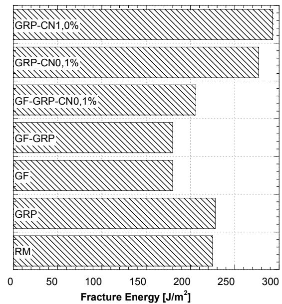
Figure 6 –Fracture energy
