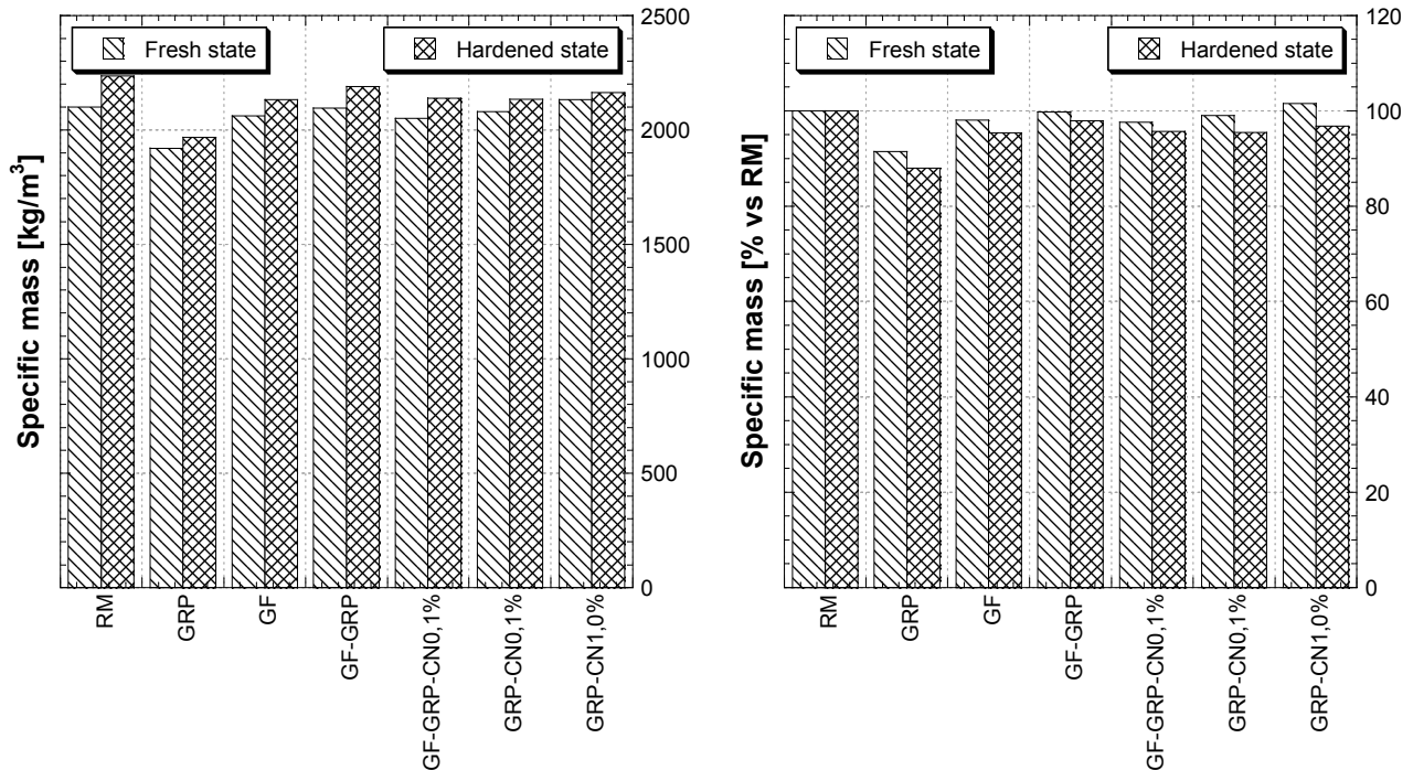
Figure 1 – Specific mass of fresh mixtures and hardened specimens (on the right the percentage variation with respect the reference mortar).
