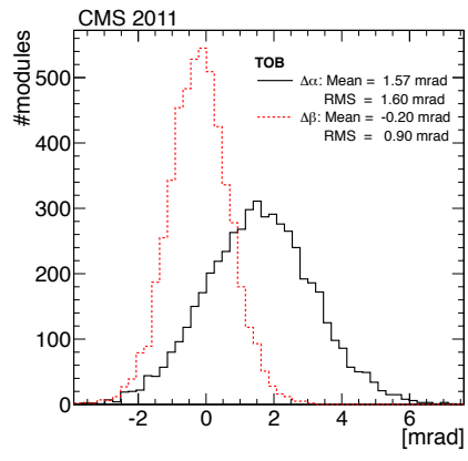
Figure 15. Distributions of the kink angles \Delta\alpha and \Delta\beta of TOB modules.
