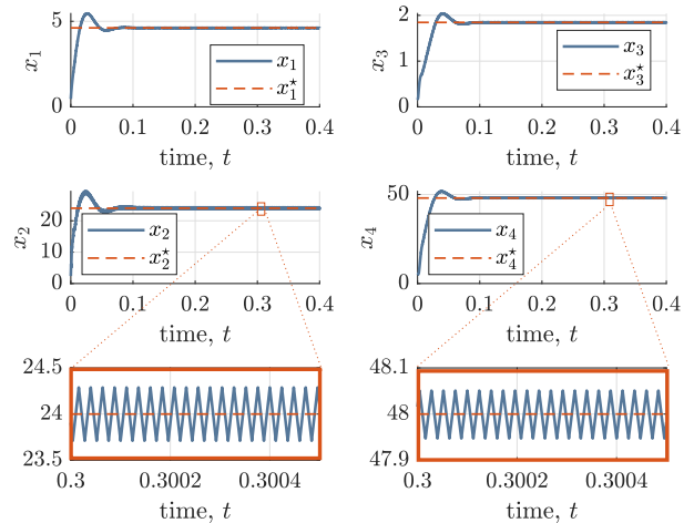
Fig. 5. Time-evolution of the boost-boost converter states. Top left: current x_1(t) . Bottom left: first stage voltage x_2(t) . Top right: current x_3(t) . Bottom right: second stage voltage x_4(t) .
