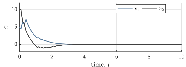
Fig. 1. Time-evolution of the state (x_1(t), x_2(t)) for the switched linear system.
