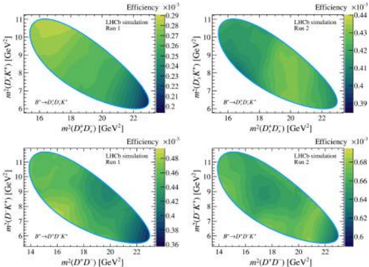
FIG. 4. Efficiency as a function of the Dalitz-plot variables for the (top) B^+ \rightarrow D_s^+ D_s^- K^+ and (bottom) B^+ \rightarrow D^+ D^- K^+ decays, calculated separately for the (left) run 1 and (right) run 2 periods.
