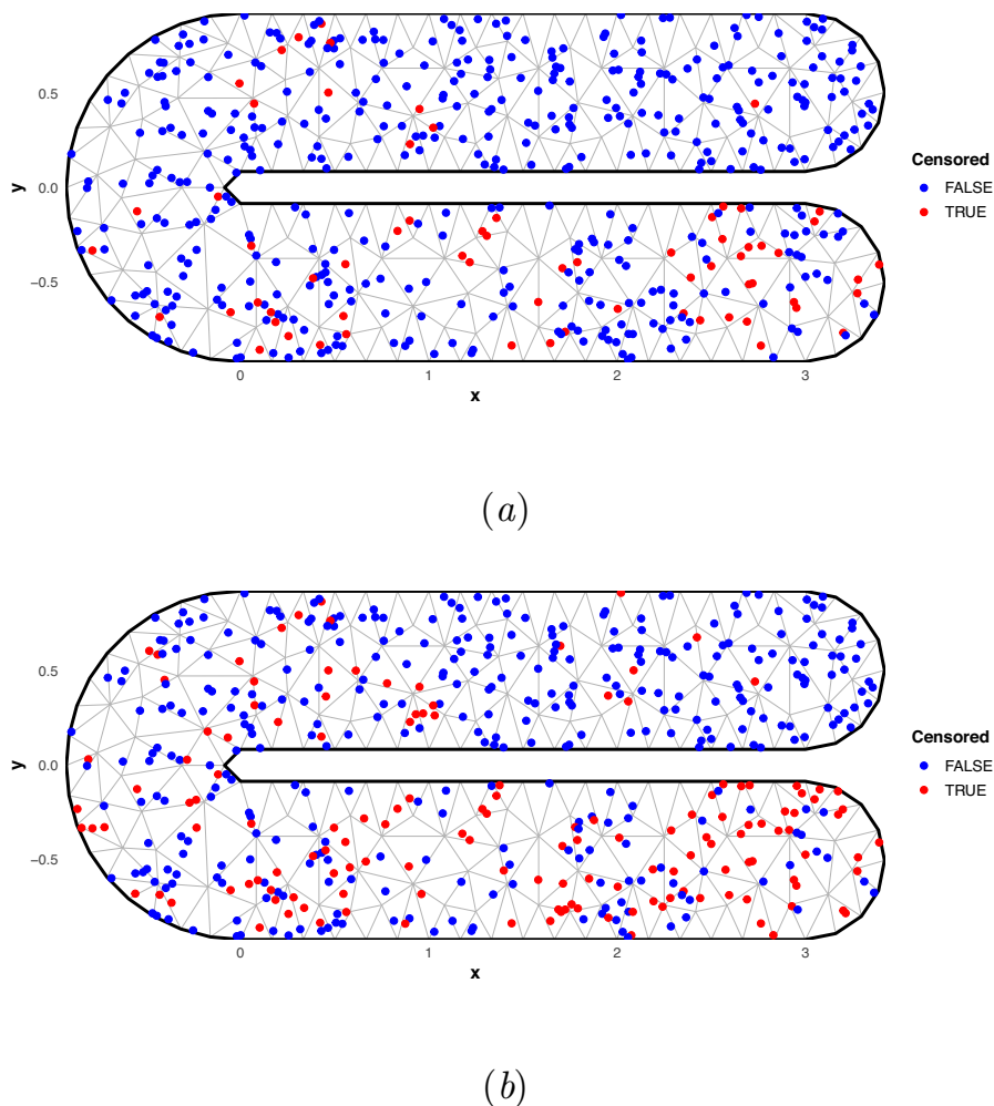
Fig. 3 Sampling design and finite element mesh for one representative replicate at n = 500 , under (a) 15% and (b) 30% censoring. Blue dots are uncensored observations, red dots are censored
