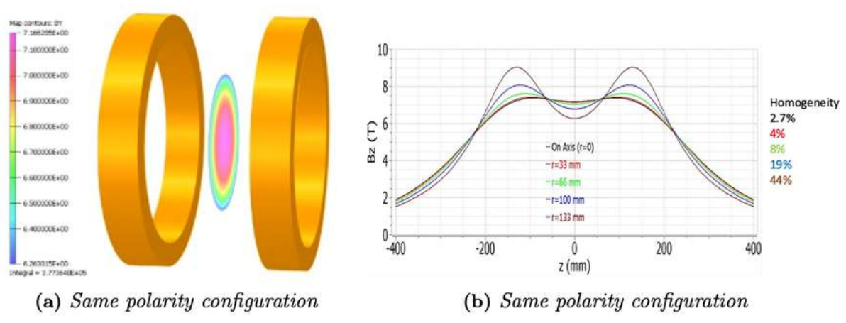
Fig. 8.6: Sketch of the split coil (without cryostat) and good field region ( \pm 200 mm).
