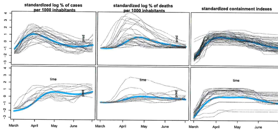
Fig. 6 COVID-19 outgrowth results of the best model, with K = 2 , L = 3 and the three random effects on. Curves belonging to each single block with superimposed the associated block specific mean curve (in light blue)
