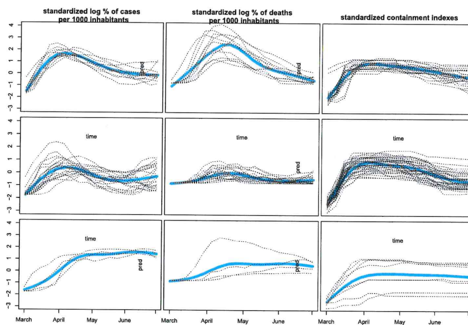
Fig. 7 COVID-19 outgrowth results of the model with K = 3 , L = 3 and the three random effects off
