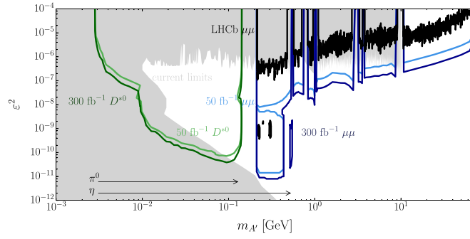
Figure 52. Current and expected limits in the dark photon parameter space mixing \epsilon^2 versus A' mass [374]. The black line represents current LHCb limits from [269], while grey-shaded regions are existing limits from other experiments. Expected limits from the proposed inclusive search with 50 and 300 \text{fb}^{-1} are shown in shades of blue. The expected sensitivity of D^{*0} \rightarrow D^0 A'(ee) at low mass is shown in shades of green. The arrows indicate the available mass range from light meson decays into e^+e^-\gamma .
