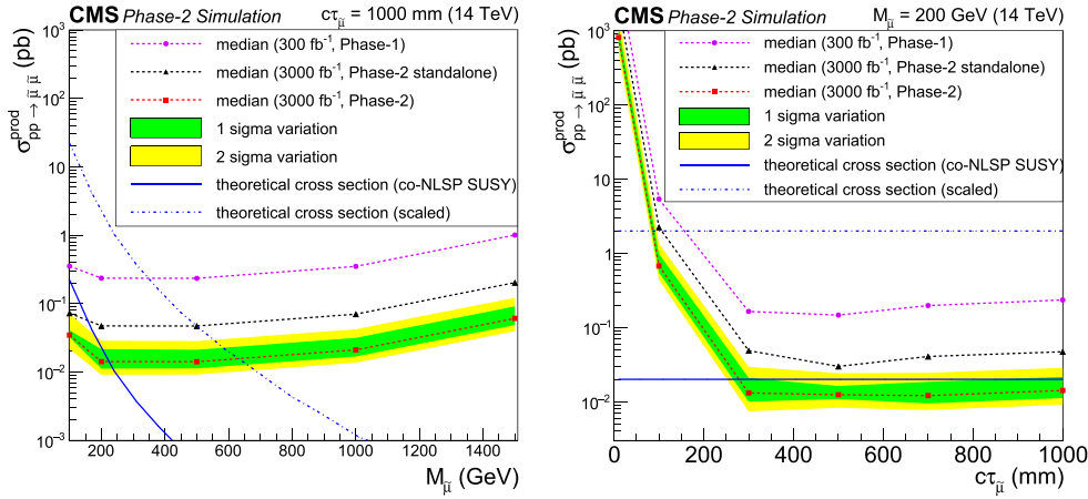
Figure 32. The 95% C.L. projected upper limits at CMS for q\bar{q} \rightarrow \tilde{\mu}\tilde{\mu}, \tilde{\mu} \rightarrow \mu\tilde{G} for various mass hypotheses for c\tau = 1 m (left), and as a function of the decay length for m_{\tilde{\mu}} = 200 GeV (right). In both panels, the theoretical cross section for the specific model is represented by the blue solid line. For different SUSY breaking scales, \tan \beta or otherwise modified parameters, the cross sections may be 100 times larger, reflected by the blue dashed–dotted line. Green (yellow) shaded bands show the one (two) sigma range of variation of the expected 95% C.L. limits. Phase 2 results with an average of 200 pile-up collisions per bunch crossing and an integrated luminosity of 300 \text{ fb}^{-1} are compared to results obtained with 300 \text{ fb}^{-1} . The black line shows the sensitivity without the DSA algorithm, which reduces the reconstruction efficiency by a factor three [350].
