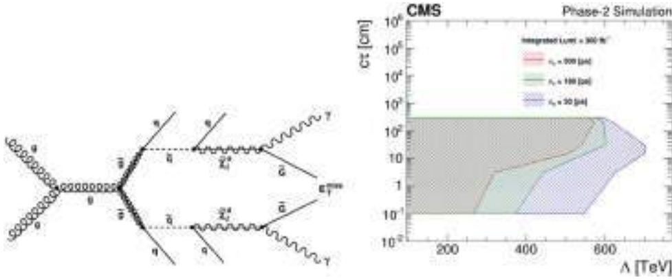
Figure 36. Left: diagrams for a SUSY process that results in a diphoton final state through gluino production at the LHC. Right: sensitivity to GMSB \tilde{\chi}_0^1 \rightarrow \tilde{G} + \gamma signals expressed in terms of neutralino lifetimes for 300, 180 and 30 ps resolution, corresponding to the current detector, the HL-LHC detector with photon timing without MTD and with MTD, respectively [351].
