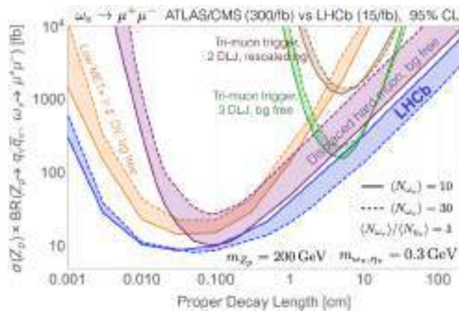
Figure 53. Projected bounds from various ATLAS/CMS searches and the LHCb search for hidden valley-like models with a Z_p decaying to a q_{HV}q_{HV} pair which then undergo hadronization in the dark sector, eventually leading to dark meson decays to di-muon final states [383].
