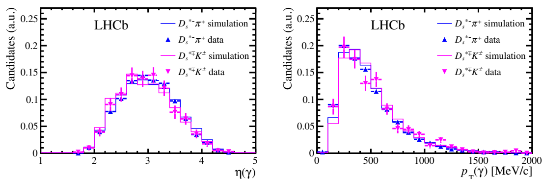
Figure 4. Distributions of (left) \eta and (right) p_T of the photons for the D_s^{*-}\pi^+ (blue) and D_s^{*+}K^+ (magenta) decays. Data, background-subtracted using the sPlot method, are represented by points, and simulations by solid lines.
