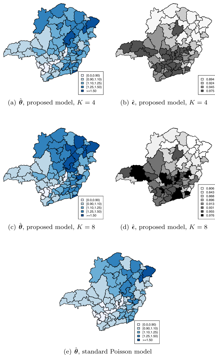
Figure 3: Posterior mean for the relative risks, \theta , of early neonatal mortality (Panels (a) and (c)) and the reporting probabilities, \epsilon , (Panels (b) and (d)) under the proposed model with K = 4 (Panels (a) and (b)) and K = 8 (Panels (c) and (d)) and the standard Poisson model (Panel (e)); Minas Gerais data, period 2009–2011.
