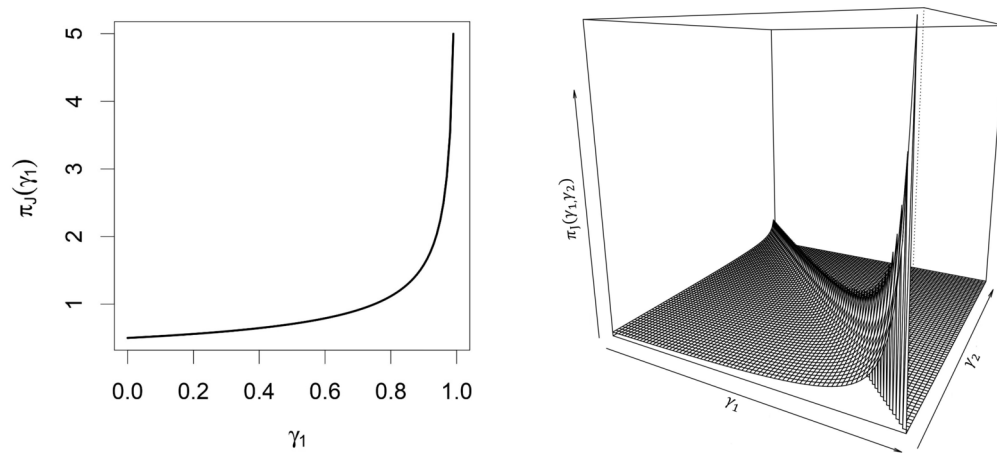
Figure 1: Marginal Jeffreys prior for \gamma_1 (left) and the joint Jeffreys prior for \gamma_1 and \gamma_2 (right).
