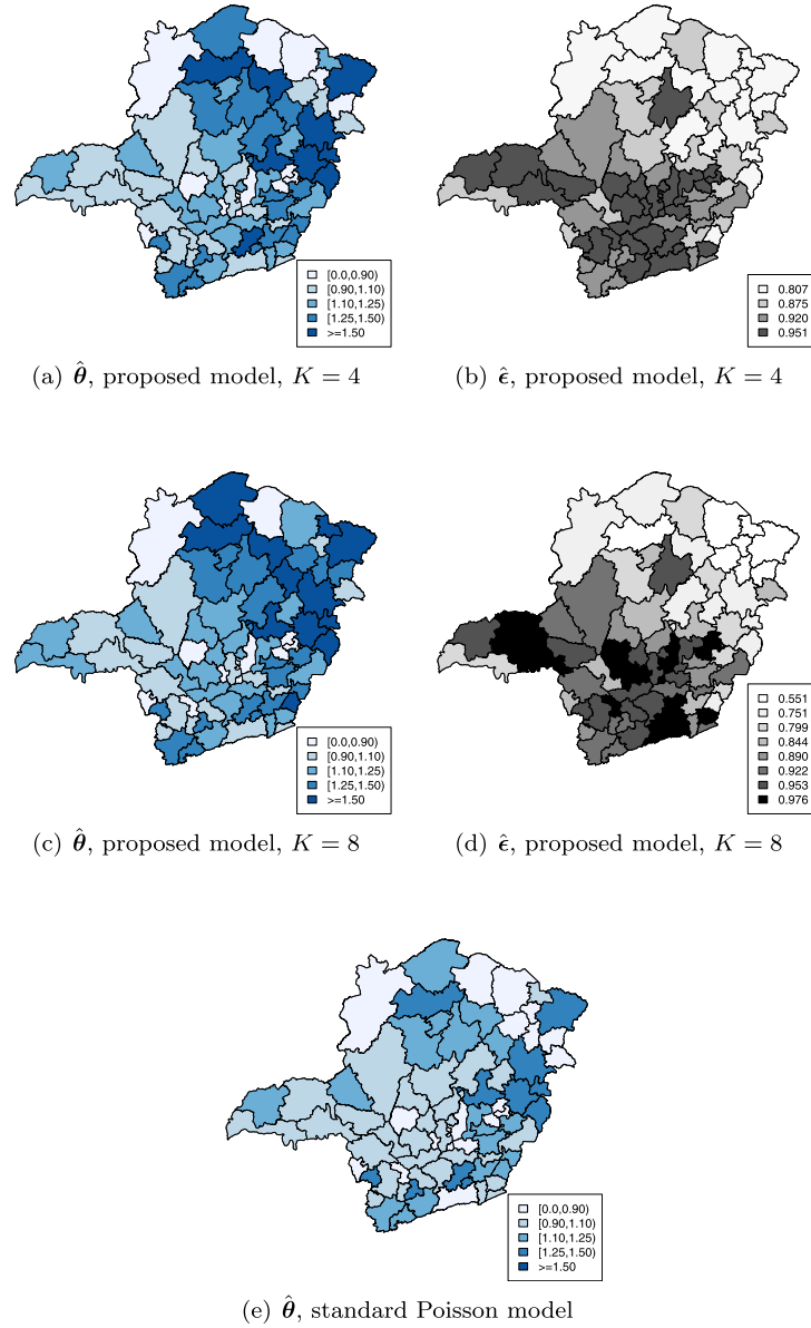
Figure 2: Posterior mean for the relative risks, \theta , of early neonatal mortality (Panels (a) and (c)) and the reporting probabilities, \epsilon , (Panels (b) and (d)) under the proposed model with K = 4 (Panels (a) and (b)) and K = 8 (Panels (c) and (d)) and the standard Poisson model (Panel (e)); Minas Gerais data, period 1999–2001.
