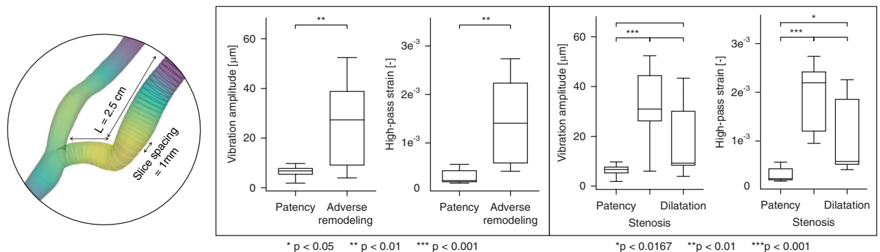
Figure 6. Boxplots illustrate differences in the distributions of time-averaged vibration amplitude and high-pass strain across groups. Cross-sectional slices from simulation results, extracted within the first 2.5 cm of the vein with 1 mm slice spacing, were used for statistical analysis. A generalized linear mixed-effects model was fitted, with Vibration amplitude and Strain as the response variables, Group (Patency, Stenosis, and Dilatation) as a fixed effect, and Patient as a random effect to account for repeated measures within individual patients. The analysis first combined all patients with adverse remodeling and then distinguished between the Stenosis and excessive Dilatation groups. For comparisons between the three groups, P values were adjusted using Bonferroni correction. The number of “*” symbols indicates the difference in levels of significance between groups.
