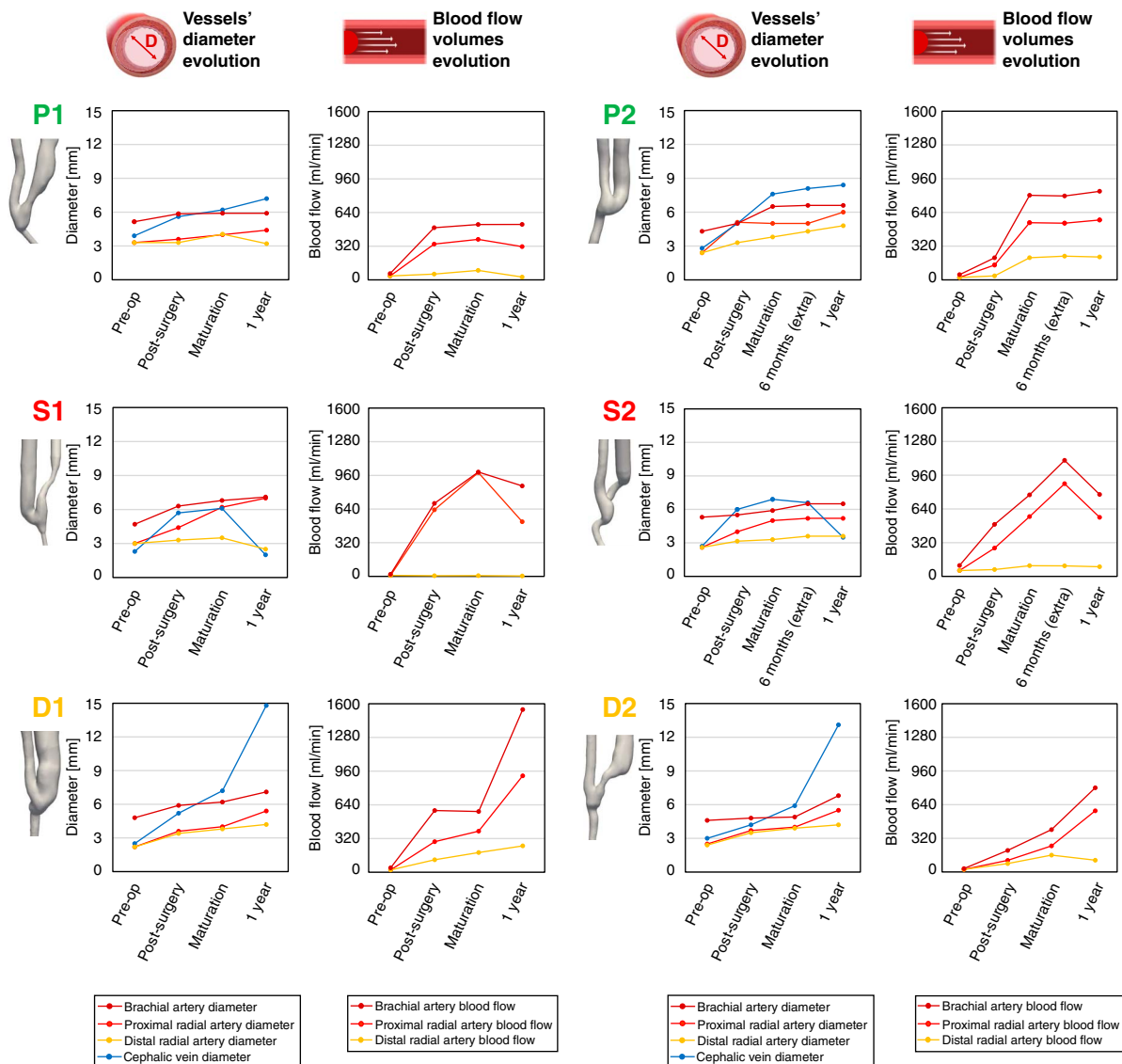
Figure 3. Evolution over time of brachial artery, radial artery (proximal and distal), and cephalic vein diameters in the six AVFs under study. The diameters of the radial artery and cephalic vein were measured approximately 2 cm from the anastomosis. The figure also illustrates blood flow volumes entering the vascular access through the brachial artery as well as through the proximal and distal radial arteries.
