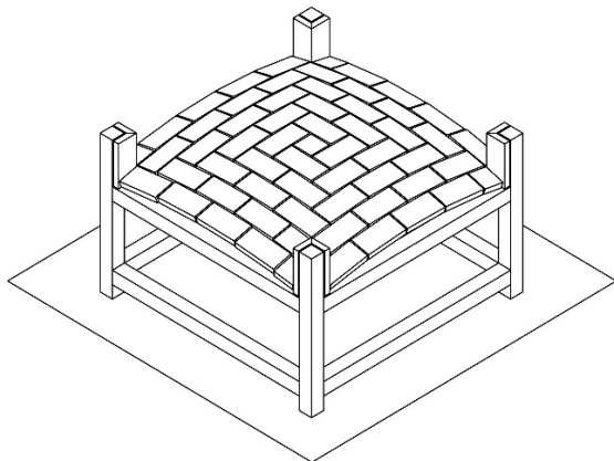
Fig. 1. The designed geometry of the lowered vault.
