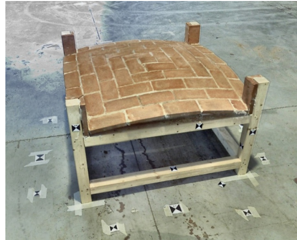
Fig. 5. Lowered vault built by T2, employing AR.
