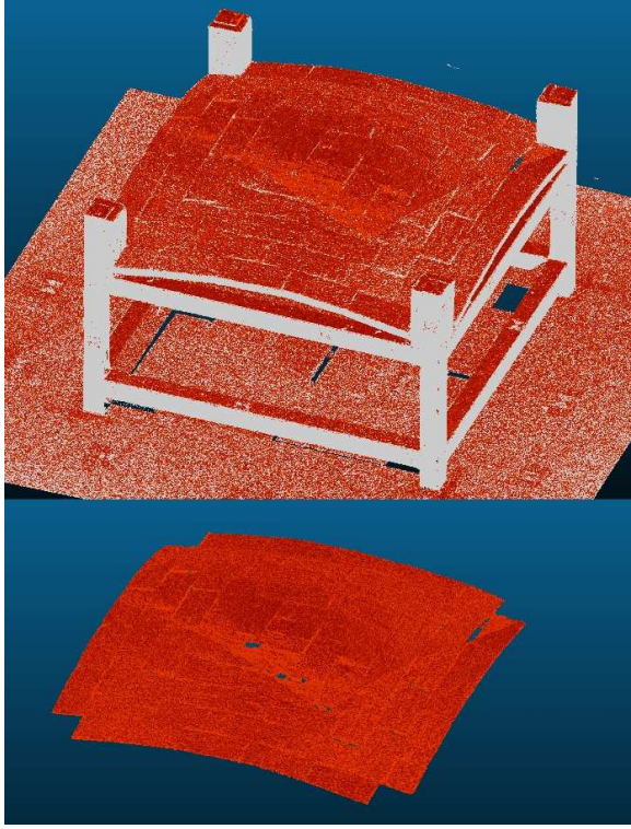
Fig. 6. PC0 of lowered vault built by T0. At the top, PC0 before the methodological cleaning process. At the bottom, PC0, after the segmentation process.
