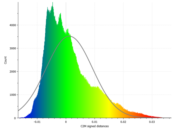
Fig. 7. Comparison of PC0 vs. designed geometry. At the top: geometrical discrepancy colour map. At the bottom: distribution of geometrical discrepancies
