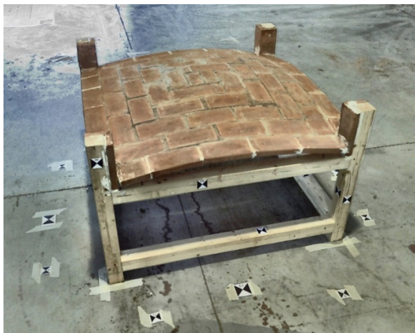
Fig. 4. Lowered vault built by T1, with the aid of a physical tracing structure.
