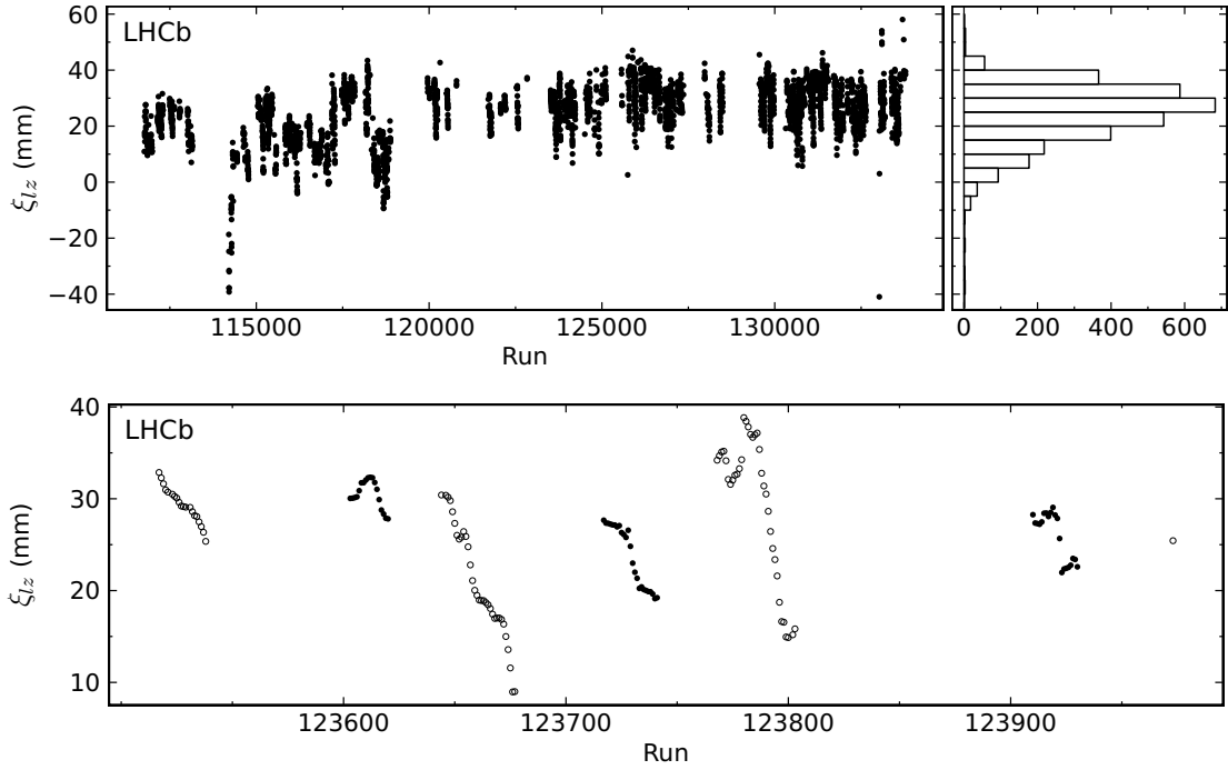
Figure 9. Longitudinal position of the luminous region \xi_{lz} during the 2012 running period. The bottom plot shows a subset consisting of a few fills (distinguished with alternating open and solid markers).
