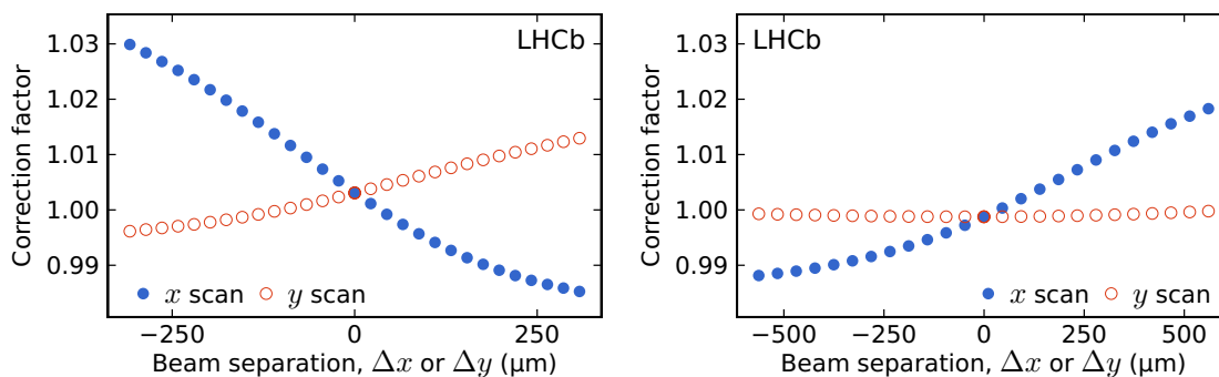
Figure 42. Efficiency correction factors for the Track observable for a scan pair in the (left) April and (right) July VDM sessions. The values for other scan pairs are similar.
