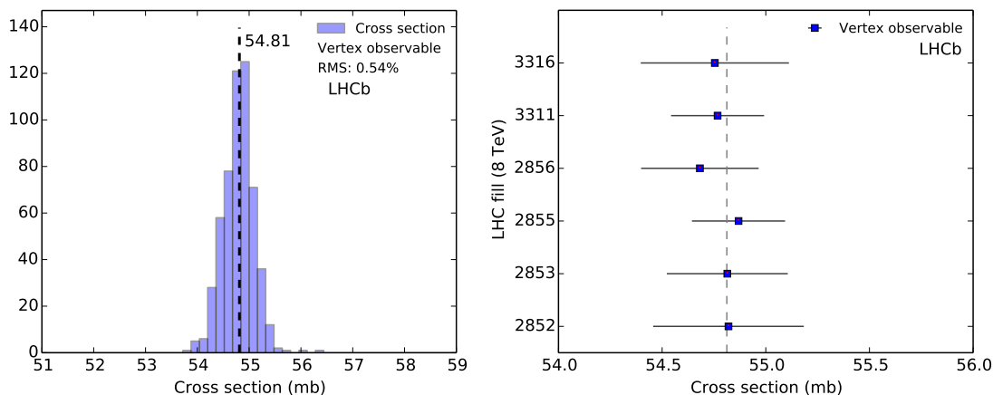
Figure 32. Overview of cross-section measurements for head-on periods in fills with \beta^* = 10 m at \sqrt{s} = 8 TeV with (left) the histogram combining all data from figure 29 and (right) the central value of cross-sections averaged per fill. The dashed vertical line indicates the median value of all measurements. The error bars indicate the standard deviation of all measurements from a fill. The statistical uncertainty of each average is smaller than the marker size.
