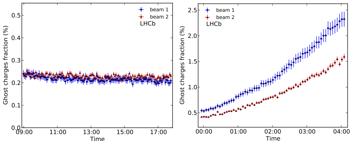
Figure 5. Ghost charge fractions for (left) fill 2855 and (right) fill 3563. Fill 2855 with \sqrt{s} = 8 \text{ TeV} shows a constant or slightly decreasing ghost charge fraction throughout the fill lasting about 9 hours. Fill 3563 ( \sqrt{s} = 2.76 \text{ TeV} ) shows an important increase of ghost charge over a period of 4 hours.
