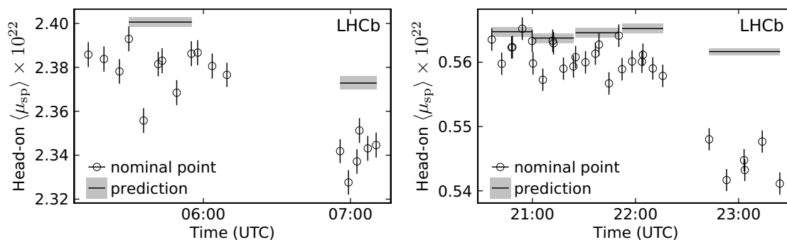
Figure 38. Evolution of the specific average number of interactions per crossing ( \mu_{\text{sp}} ) at the nominal head-on beam positions during the (left) April and (right) July VDM sessions. In each scan the nominal point was measured three times and the average over bunches is plotted with open markers. The value at the actual zero beam separation is predicted for each scan pair (excluding offset and tilted scans) and shown with a horizontal band. The difference with respect to the values at zero nominal separation is due to the working point not being exactly at zero beam separation. The beam positions were not re-optimized during the sessions.
