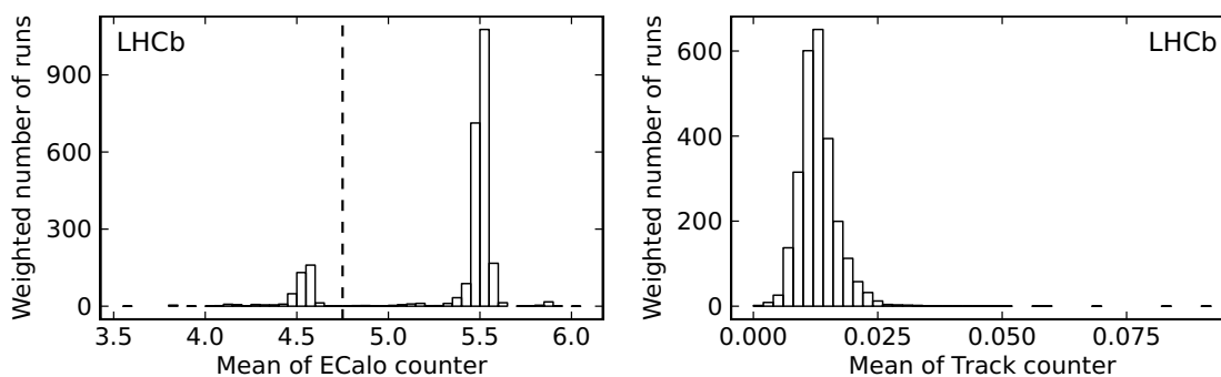
Figure 6. Mean value of (left) ECalo and (right) Track observables in ee crossings. Each histogram entry represents the average over a run 2 in 2012 and is weighted with the corresponding integrated luminosity. For measurements using the ECalo and Calo observables we discard the runs for which the ECalo pedestal mean is lower than 4.75 (dashed vertical line).
