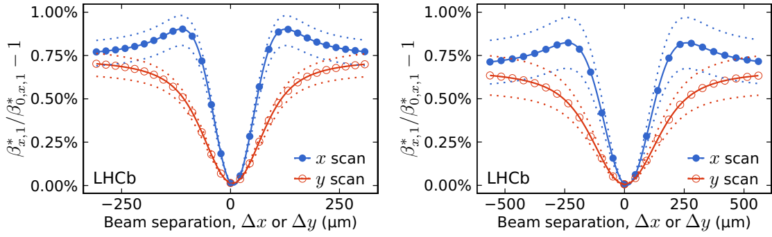
Figure 45. Relative \beta^* change for beam 1 in the x axis as a function of beam separation for a scan pair in the (left) April and (right) July VDM sessions. The values for other scan pairs are similar. The values for beam 2 are similar owing to similar bunch intensities. The values for the y axis are also similar with x and y scans exchanged. The markers and the solid line represent the average, while the dotted lines correspond to the extremes among colliding bunches. The reference \beta^* is chosen such that the relative change is zero at the separation corresponding to maximum luminosity.
