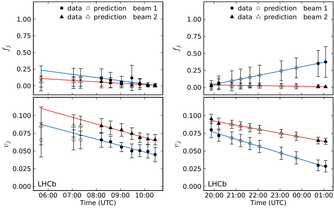
Figure 48. Values of the (top) factorizability parameter f_j and (bottom) generic factorizability measure v_j in the (left) April and (right) July VDM sessions. The filled markers and the corresponding error bars indicate the average and the RMS of BGI measurements for individual bunch pairs. In the case of the July scans, BGI measurements are available before and after the VDM session, thus the values are linearly interpolated to obtain predictions at the time of VDM scan pairs (open markers). For April, as BGI data are only available after the VDM scans, the closest data points are used as a prediction, while the difference to the linear extrapolation is added in quadrature to the uncertainties. The trend of the generic factorizability measure shows that beam distributions become more factorizable as function of time.
