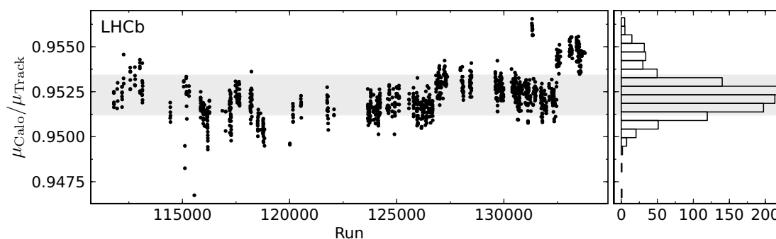
Figure 14. Ratio of the relative luminosities using the Track and the Calo observables during the 2012 running period. Only data for runs that are longer than 30min are plotted. The variation of the ratio after subtraction of the variation due to statistical fluctuations is shown with a shaded area spanning \pm 1\sigma around the mean.
