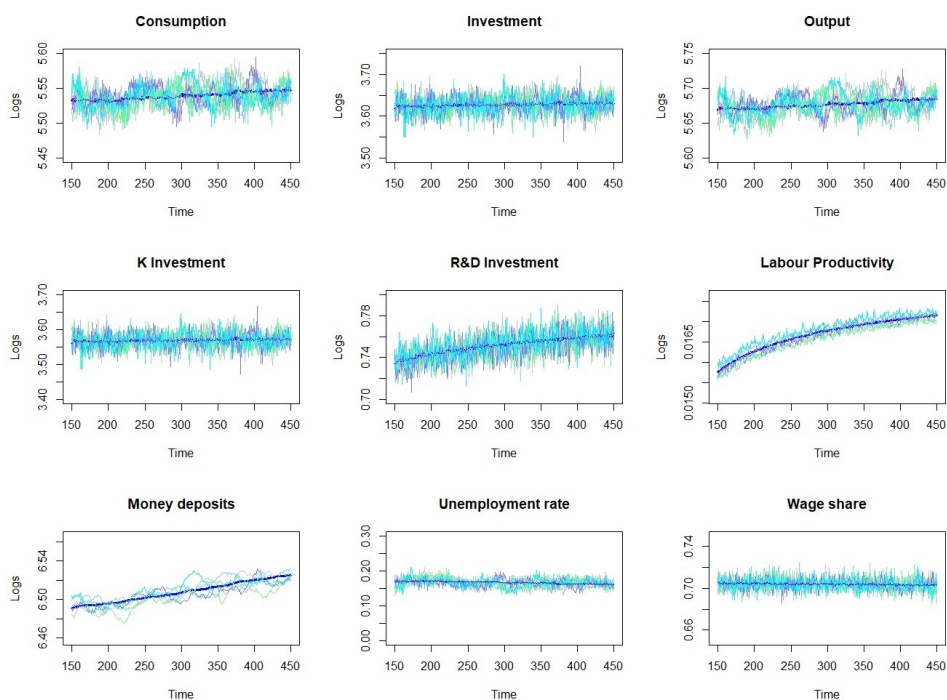
Figure 2.4. Baseline model: single Monte Carlo runs
