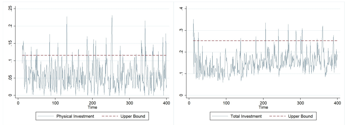
Figure 3.4. Investment heterogeneity
