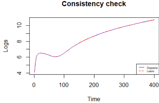
Figure 3.7. Stock-flow consistency check on selected simulation
