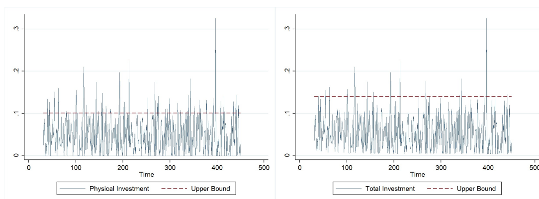
Figure 2.13. Investment lumpiness?
