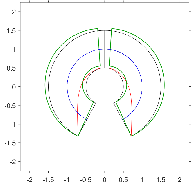
Fig. 25. Least-thickness collapse mechanism, with line of thrust and line of friction: purely-overturning at \mu \rightarrow \infty ( \varphi = 90^\circ ): \alpha = 2.786498150651177 \simeq 159.7^\circ ( A = 1/2 , \eta = 2 ) (top); \alpha = 2.648388899151005 \simeq 151.7^\circ ( A = 2/3 , \eta = 1 ) (low).
