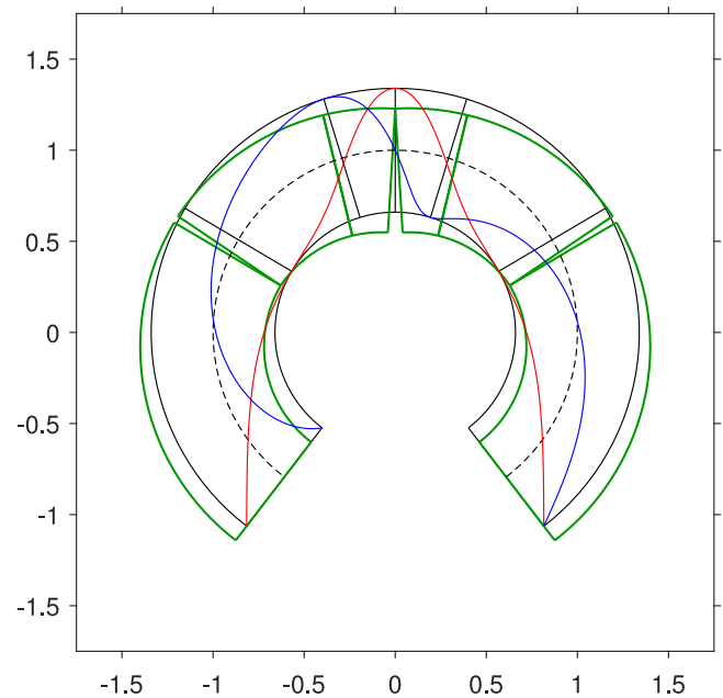
Fig. 19. Least-thickness collapse mechanism, with line of thrust and line of friction: at “Triple point” with \alpha_T = 2.487161163767182 \simeq 142.5^\circ , \mu_T = 1.415270827756885 ( \varphi_T \simeq 54.8^\circ ), \eta_T = 0.6796047320988855 : rotational-sliding (top); sliding-rotational (low).
