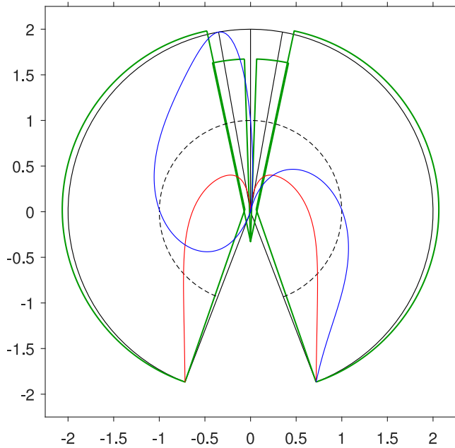
Fig. 24. Least-thickness collapse mechanism, with line of thrust and line of friction: at “Border point” with \alpha_B = 2.774176793356033 \simeq 158.9^\circ , \mu_B = 2.690297881776621 ( \varphi \simeq 69.6^\circ ), \eta_B = 2 : purely-sliding (top); overturning-sliding (low).
