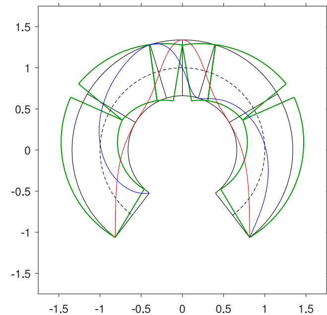
Fig. 18. Least-thickness collapse mechanism, with line of thrust and line of friction: at “Triple point” with \alpha_T = 2.487161163767182 \simeq 142.5^\circ , \mu_T = 1.415270827756885 ( \varphi_T \simeq 54.8^\circ ), \eta_T = 0.6796047320988855 : purely-sliding (top); purely-rotational (low).
