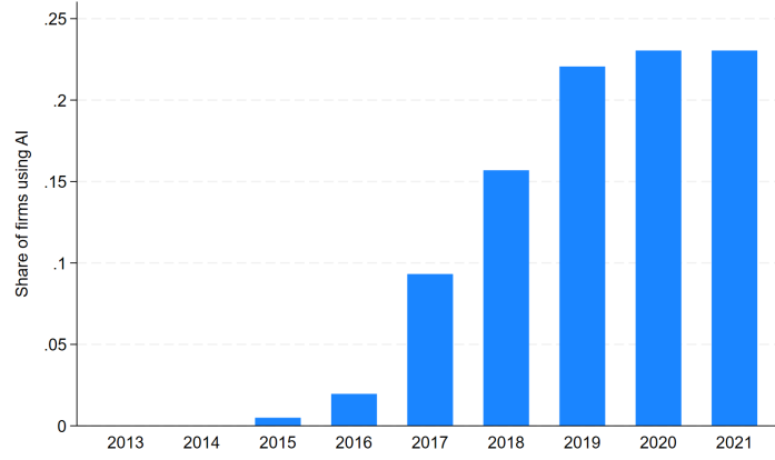
Figure 2.2: Firms entering the treatment status and remaining treated
