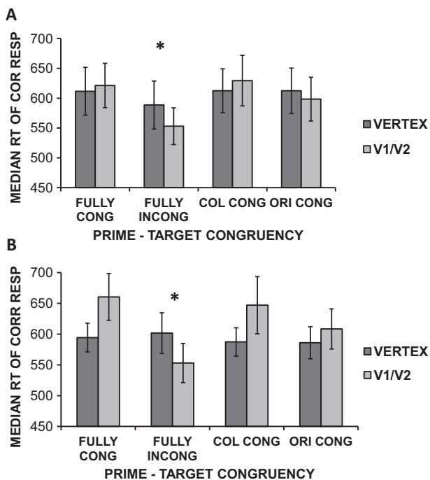
Fig. 2. Mean ( n = 16 ) of the median RTs (milliseconds) of correct responses as a function of TMS site and prime-target congruency in Experiment 1 for subthreshold (panel A) and suprathreshold (panel B) TMS. In Experiment 1, TMS was applied at target onset. For both TMS intensities, V1/V2 TMS facilitated performance of fully incongruent trials (relative to Vertex TMS) while having no significant effect on either fully congruent, color congruent or orientation congruent trials. Errors bars indicate \pm 1 SEM.
