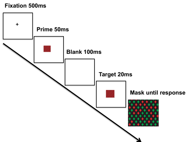
Fig. 1. Timeline of an experimental trial. On each trial, participants were presented with a prime that was either a red–black or green–black grating, tilted either clockwise or counterclockwise. This was followed by a target which could be either fully congruent with the prime (i.e. the same stimulus), fully incongruent (i.e. both color and orientation differed), or partially congruent (either color or orientation matched the prime). Participants had to indicate the color of diagonals of the stimulus target (red or green). In this figure, a fully congruent trial (i.e. prime and target matched for both color and orientation) is depicted. In Experiment 1, Single-pulse TMS was delivered at target onset over either V1/V2 region or over the Vertex (baseline) at either 80% or 120% of participant’s PT. In Experiment 2, single pulse of TMS was applied at 100 ms after stimulus onset. (For interpretation of the references to color in this figure legend, the reader is referred to the web version of this article.)
