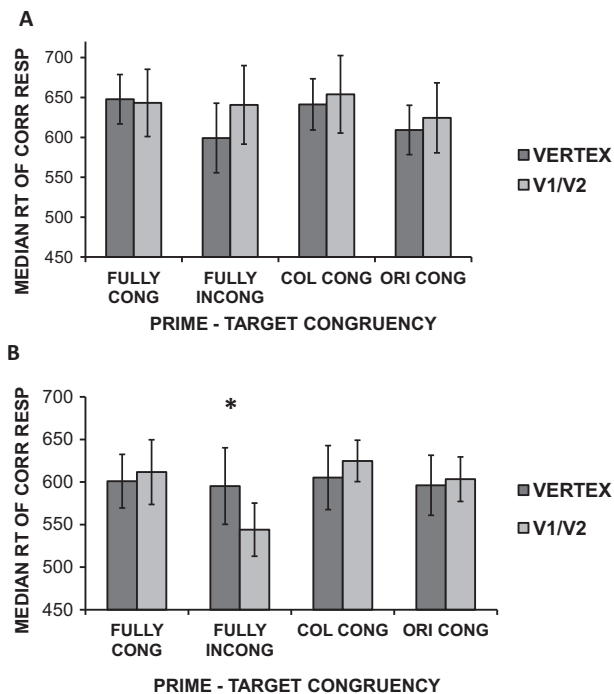
Fig. 3. Mean ( n = 17 ) of the median RTs (milliseconds) of correct responses as a function of TMS site and prime-target congruency in Experiment 2 for subthreshold TMS (panel A) and suprathreshold TMS (panel B). In Experiment 2, TMS was applied 100 ms after target onset. With suprathreshold TMS, V1/V2 TMS facilitated performance of fully incongruent trials (relative to Vertex TMS) while having no significant effect on either fully congruent trials, color congruent or orientation congruent trials. Subthreshold TMS had no effects on any target type. Error bars indicate \pm 1 SEM.
