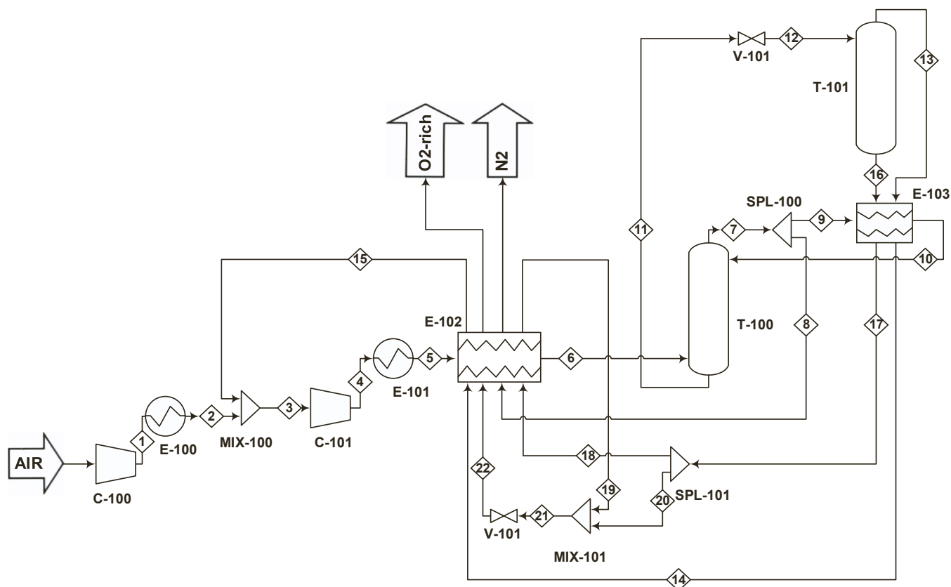
Fig. 4. N 2 separation process.
