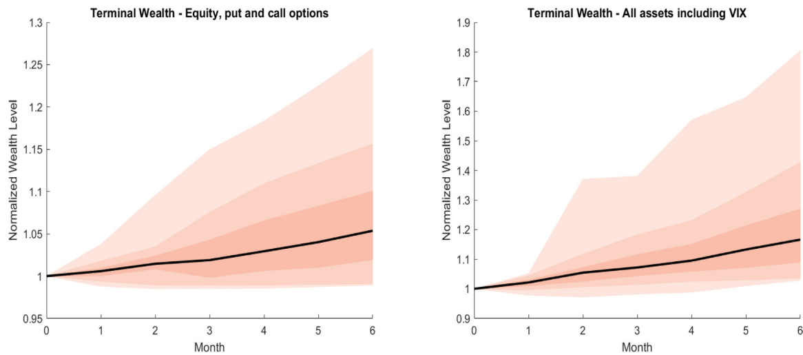
Fig. 12. Optimal wealth evolutions with h = 6 : long call and put free investment opportunities in period 3 with only equity i = 1 or all assets and the VIX i = 4 : \mathcal{L}(0.5, C_{jATM}^6, \mathcal{I}_i, 3) .
