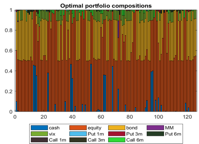
Fig. 18. Monthly replicating portfolio composition in the out-of-sample period (Jan 2011–Jun 2021 in the x-axis span from 0 to month 126 with monthly steps). \mathcal{L}(0.5, C_{j,ATM}^6, \mathcal{I}_4) with 10% upper bound on VIX and 50% lower bound on equity.
