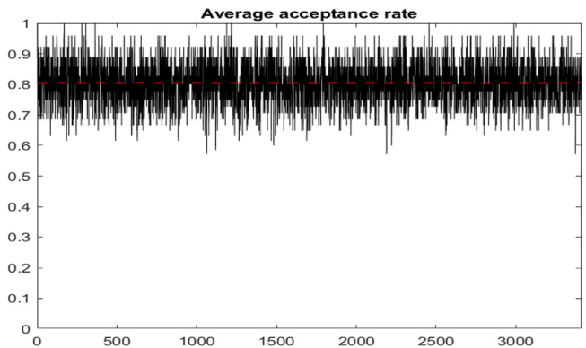
Fig. 2. Average acceptance rate (red dashed line) and node specific acceptance rate computed for 10 – 4 5 scenario tree. All results are averages over 40 independent experiments. (For interpretation of the references to color in this figure legend, the reader is referred to the web version of this article.)
