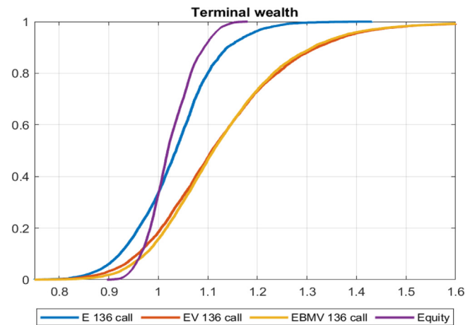
Fig. 7. Covered call strategy \mathcal{L}(0, C_{j,ATM}^2, \mathcal{I}_i, 2) with t_j = \{1, 3, 6\} short ATM call position and i = 1, 2, 4 with \lambda = 0 . Terminal wealth distributions for an equity portfolio with no options, h = 0 ("Equity" cdf), and cdf's associated with the canonical covered call ( h = 1 ), plus volatility ( h = 2 ) and plus the other assets ( h = 4 ), "E 136 call", "EV 136 call" and "EBMV 136 call", respectively.
