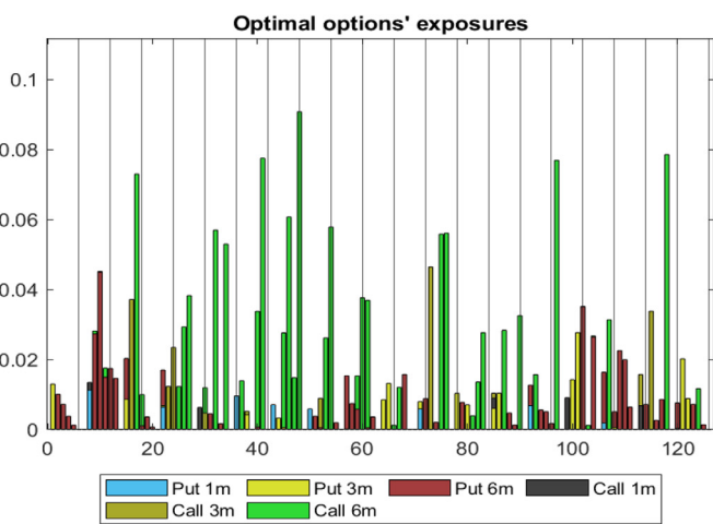
Fig. 17. Top: Optimal wealth evolutions for different strategies over the semesters in the out-of-sample period (Jan 2011–Jun 2021). We denote the wealth trajectories \mathcal{L}(0.5, C_{j,ATM}^6, \mathcal{I}_4) with Opt50E10V, \mathcal{L}(0.5, C_{j,ATM}^6, \mathcal{I}_4) with NoOpt50E10V, with Fix-Mix(60 – 40 equity-bond), 1/N, and Bond and S&P500 for the Equity. Bottom: Optimal option positions for each semester in the out-of-sample period (Jan 2011–Jun 2021). \mathcal{L}(0.5, C_{j,ATM}^6, \mathcal{I}_4) with long ATM Put and Call with maturity t_j = 1, 3, 6 .
