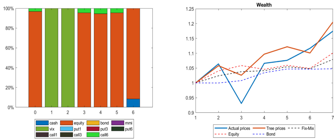
Fig. 16. Optimal portfolio compositions(left-hand-side) and corresponding wealth evolution (right-hand-side) along the replicating scenario for the test problem \mathcal{L}(0.5, C_{j,ATM}^6, \mathcal{I}_4, 3) , t_j = \{1, 3, 6\} and m = 3 .
