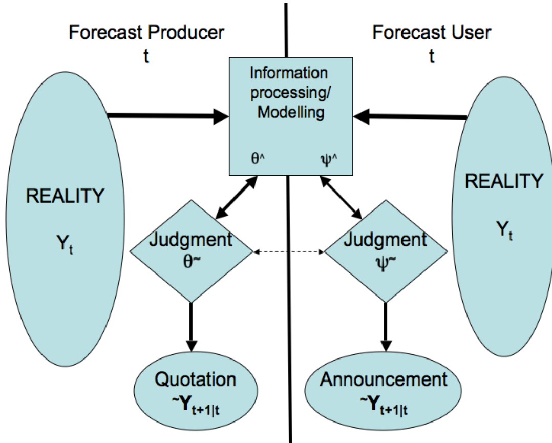
Figure 1: A synopsis of the classical forecasting environments
