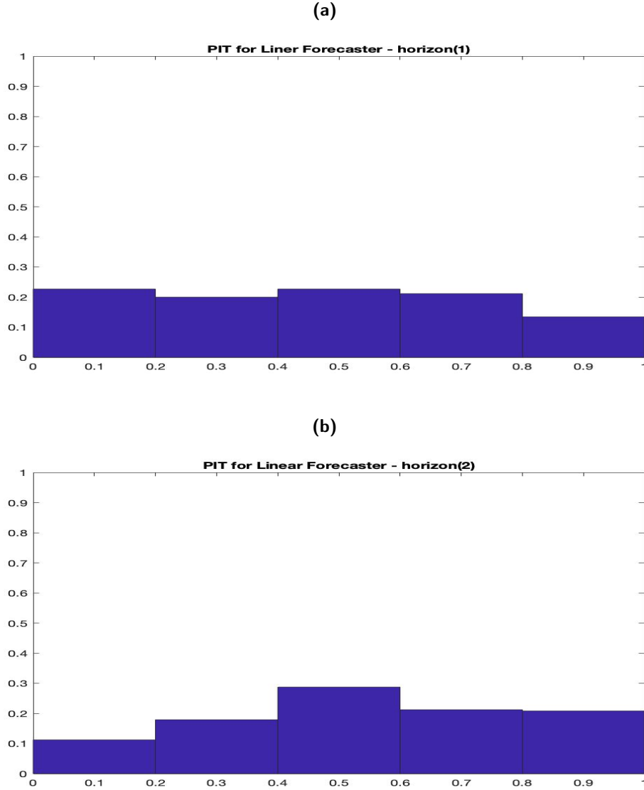
Figure 3: The problem of Misspecification due to Strategic Judgment (Example 1)
