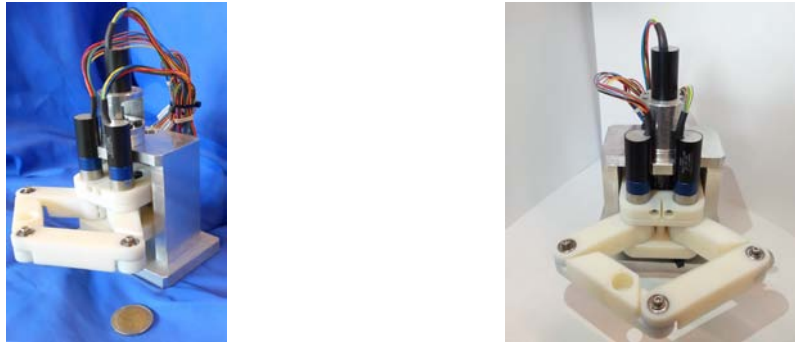
Figure 3: two views of the manipulator's physical prototype
