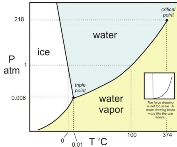
Figure 11: Water phase diagram.
