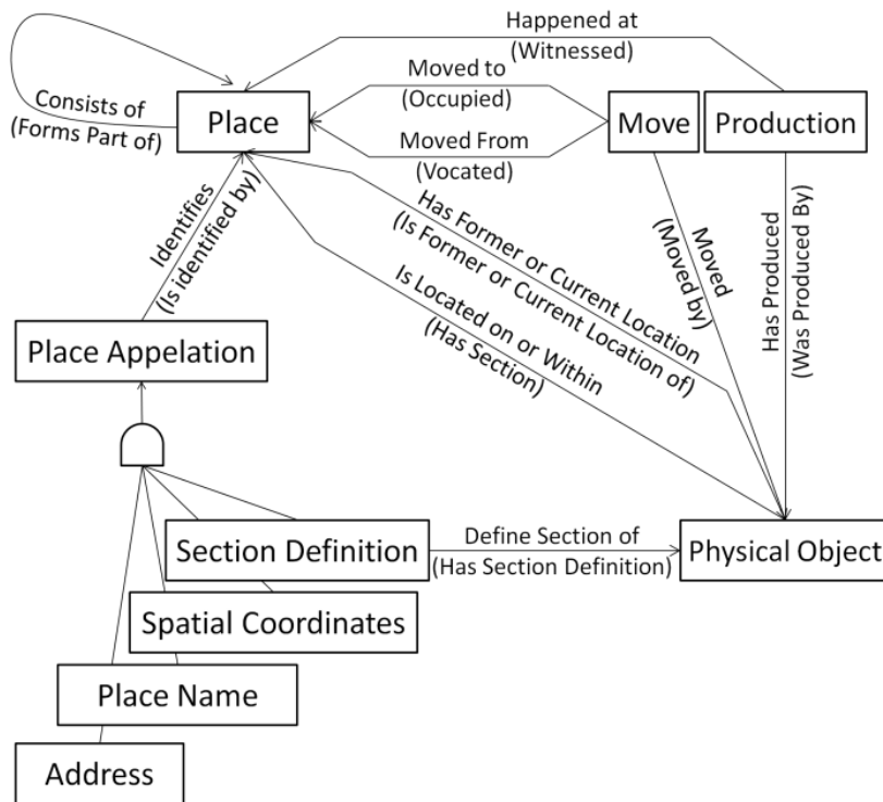
Figure 4: Space ontology.
