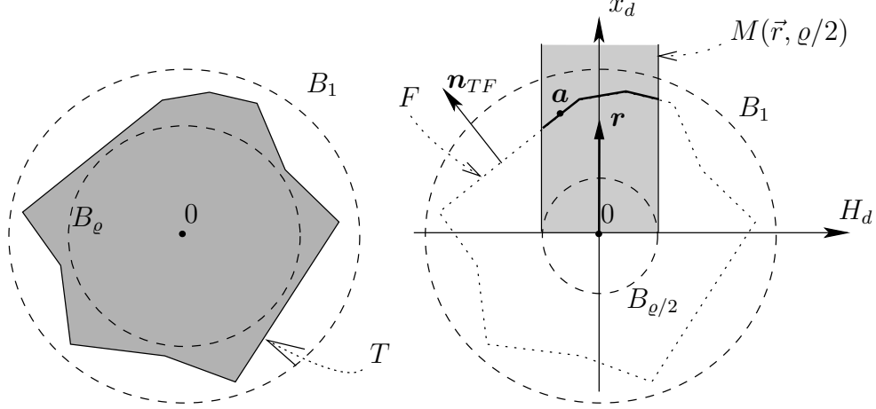
Figure A.7: Illustration of the proof of Lemma 22
