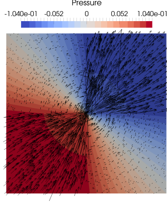
Figure 6: Solution (53) (Darcy problem with discontinuous permeability). Arrows indicate orientation and magnitude of the velocity at a given point.
