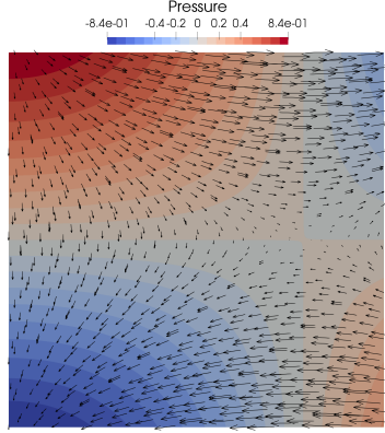
Figure 3: Solution (51) with (\mu, \nu) = (1, 1) (Brinkman problem). Arrows indicate orientation and magnitude of the velocity at a given point.
