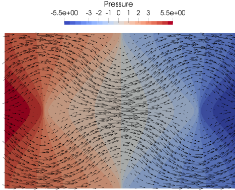
Figure 5: Solution (52) (Darcy problem with variable permeability). Arrows indicate orientation and magnitude of the velocity at a given point.
