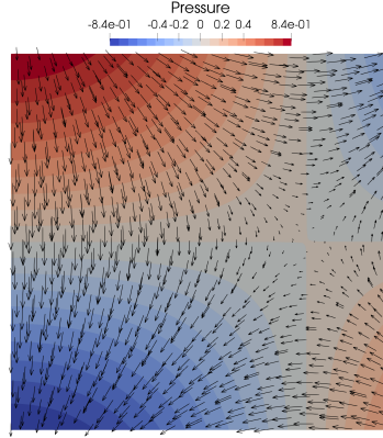
Figure 2: Solution (51) with (\mu, \nu) = (0, 1) (Darcy problem). Arrows indicate orientation and magnitude of the velocity at a given point.
