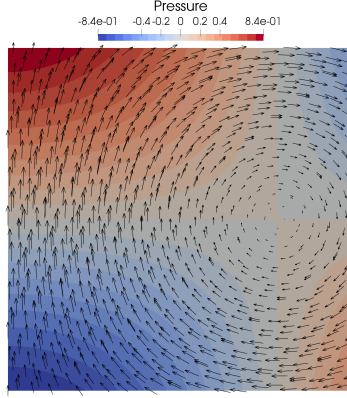
Figure 4: Solution (51) with (\mu, \nu) = (1, 0) (Stokes problem). Arrows indicate orientation and magnitude of the velocity at a given point.
