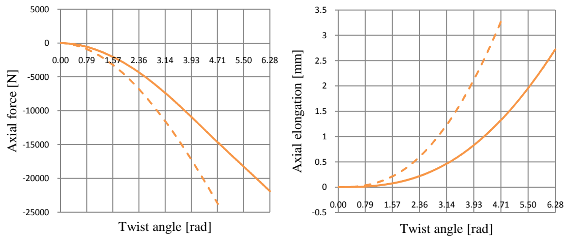
Figure 6. Swift effect outcomes for tubular (dotted lines) and solid (solid lines) specimens (linear kinematic hardening case).
