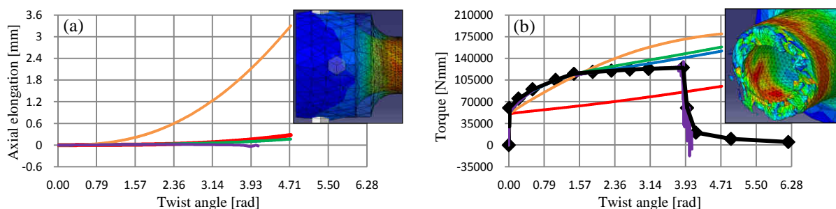
Figure 1. FEM numerical results: (a) Outcome of the Swift effect; (b) Torsion response up to fracture.
