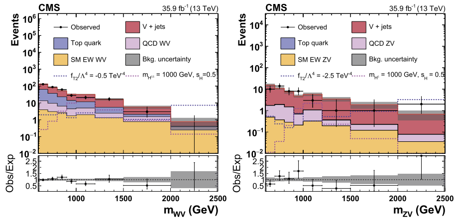
Fig. 4. Distributions of m_{WV} (left) and m_{ZV} (right) in the signal region. The gray bands include uncertainties from the predicted yields. The histograms for other backgrounds include the contributions from QCD VV, top quark, W+jets, and Drell–Yan processes. The predicted yields are shown with their best-fit normalizations from the background-only fit. The dashed lines show the signal predictions for two aQGC parameters, and charged Higgs bosons in the GM model. The overflow is included in the last bin. The bottom panel in each figure shows the ratio of the number of events observed in data to that of the total background prediction.
