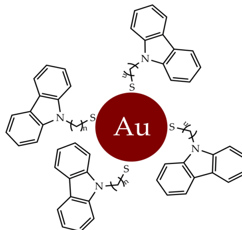
Figure 2. Gold nanoparticles functionalized with N -thioalkylcarbazole derivatives.
