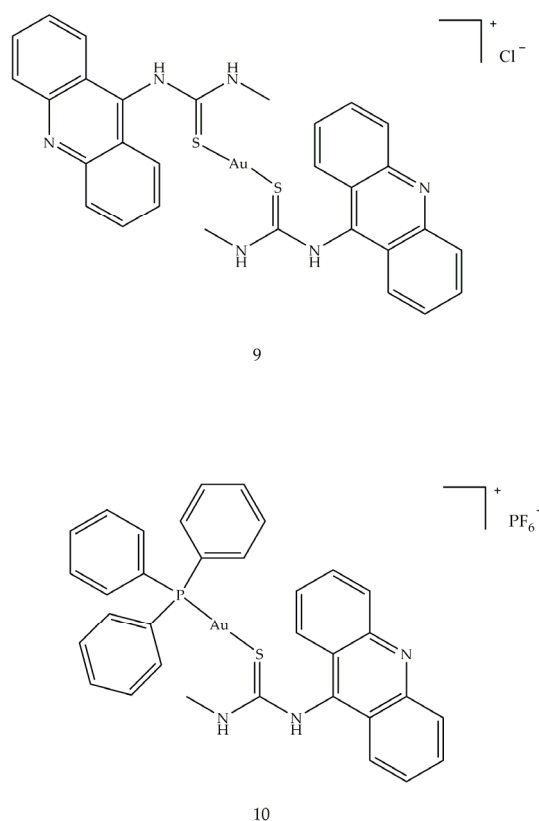
Figure 11. Molecular structure of acridine thiourea gold (I) (9 and 10).
