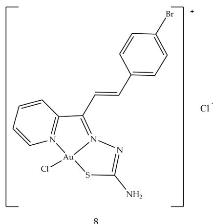
Figure 6. Molecular structure of the gold (III) thiosemicarbazone (8).
