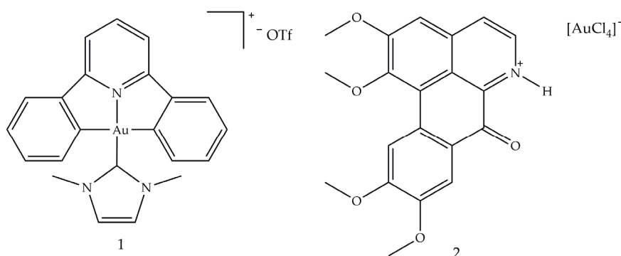
Figure 3. Molecular structure of [\text{Au}(\text{C}^{\wedge}\text{N}^{\wedge}\text{C})(\text{Ime})]\text{CF}_3\text{SO}_3 (1) and [\text{OGH}][\text{AuCl}_4] (2) [60].
