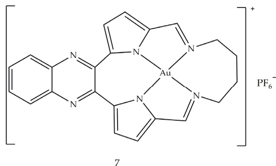
Figure 5. Molecular structure of the gold (III) macrocycle (7) [60].
