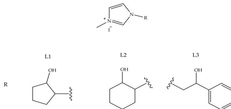
Figure 7. NH-Carbene proligands L1, L2 and L3, employed in AuL n ( n = 1-3 ) complexes.
