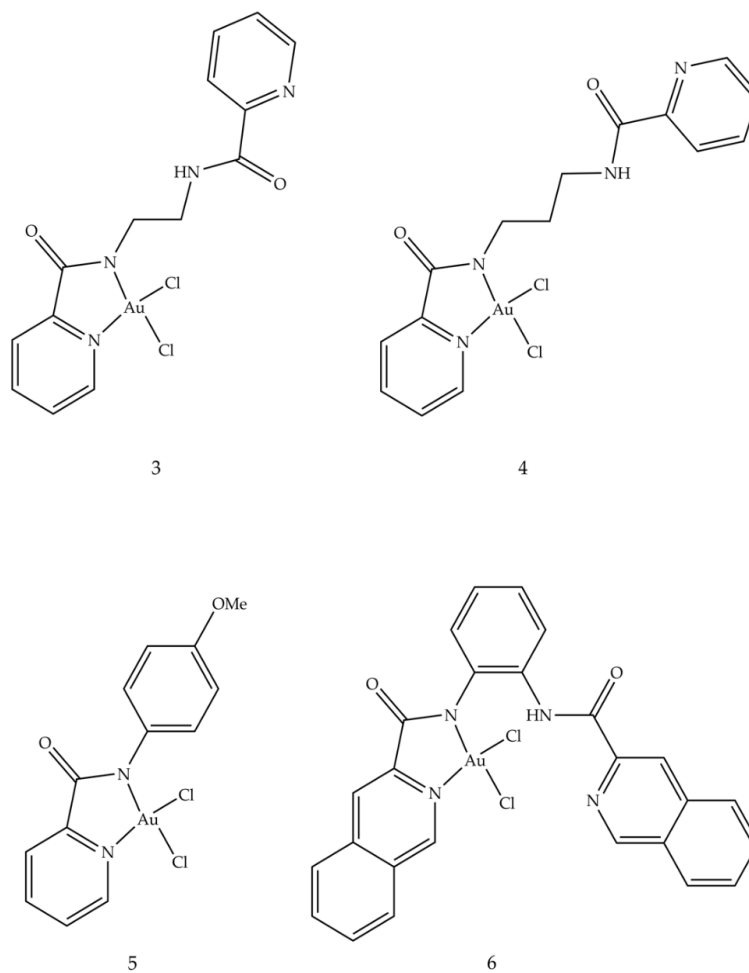
Figure 4. Molecular structures of gold (III) pyridyl and isoquinolylamido chelates (3–6) [60].
