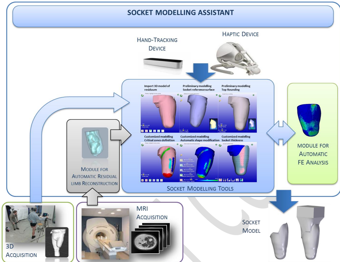
Fig 2: SMA architecture.
