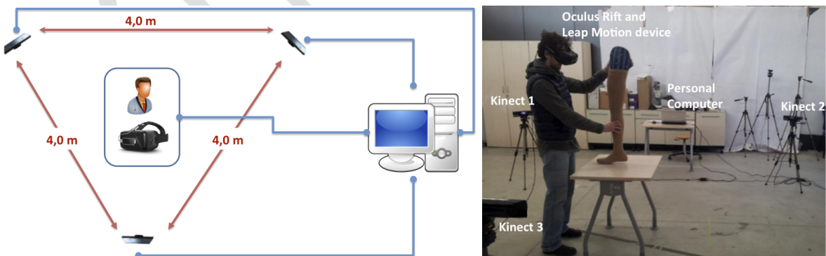
Fig. 3: VOLAB Hardware architecture.
