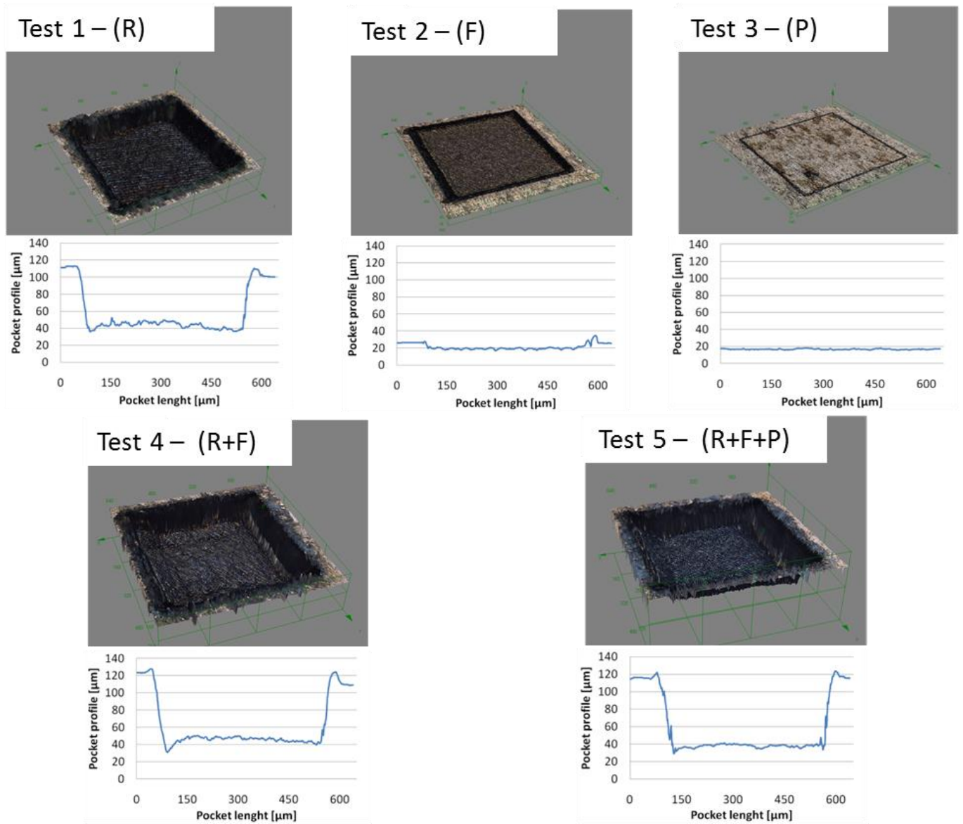
Figure 4. Single and cumulative laser cycle profiles (No gas tests)
