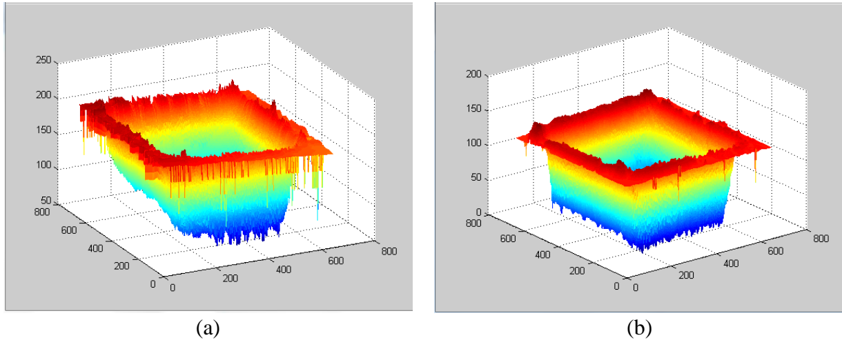
Figure 5. Qualitative comparison between Test 10(a) and Test 11 (b).
