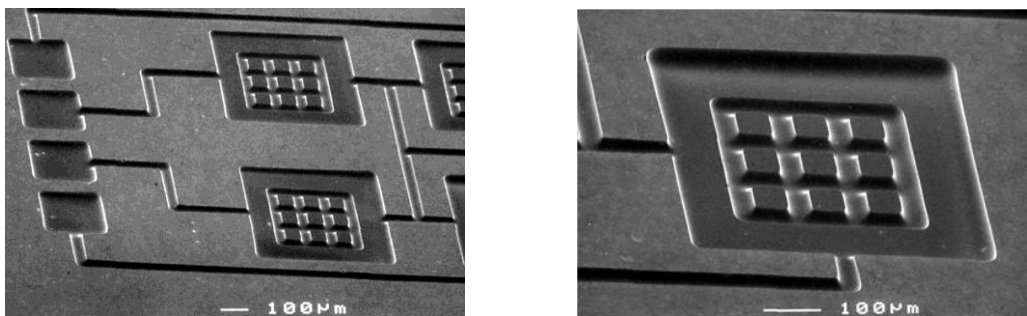
Figure 1. Two-level titanium microstructure designed for micro-fluidic applications [8]
