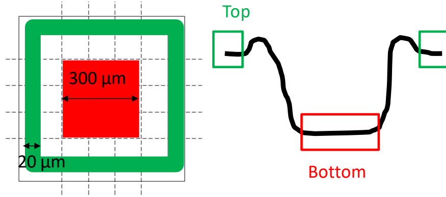
Figure 3. Strategy adopted for the pocket geometry acquisition.
