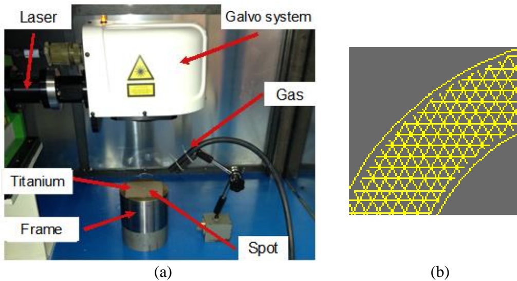
Figure 2. (a) Set up of the experiments, (b) laser path net three line filling strategy
