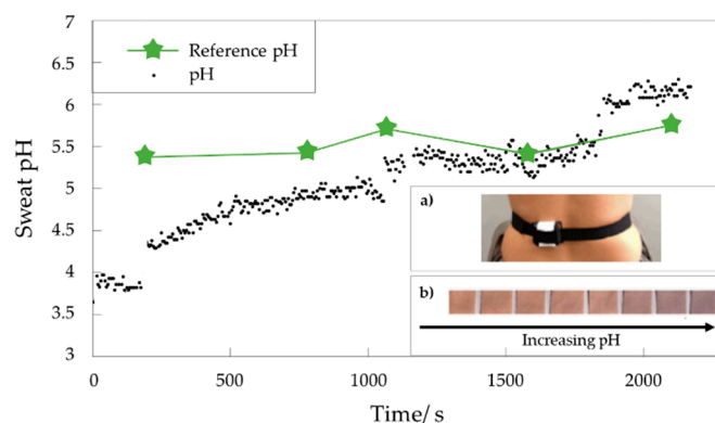
Figure 3. Comparison of sweat pH measurements carried out by wearable sensors and a reference pH meter as a function of time. In insets, the on-body position of the device during physical activities (a) and colour changing as a function of increasing pH values (b). Adapted with permission from [56] Copyright (2016) American Chemical Society.
