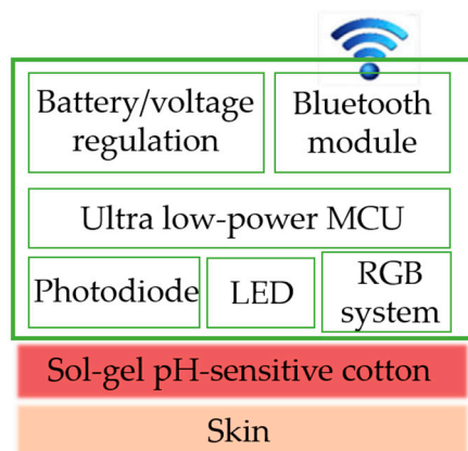
Figure 2. Block diagram of smart halochromic sensor.
