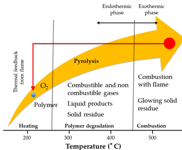
Figure 6. Schematic representation of polymer combustion process.
