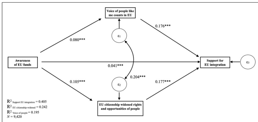
Figure 2. Standardised estimates for awareness of EU social programmes and support for the EU with correlated errors. Note: N= 9420. The significance levels shown here are for the unstandardised solution. * p < .05 , ** p < .01 , *** p < .001 . Coefficients of control variables are available in the Appendix Table A4.
