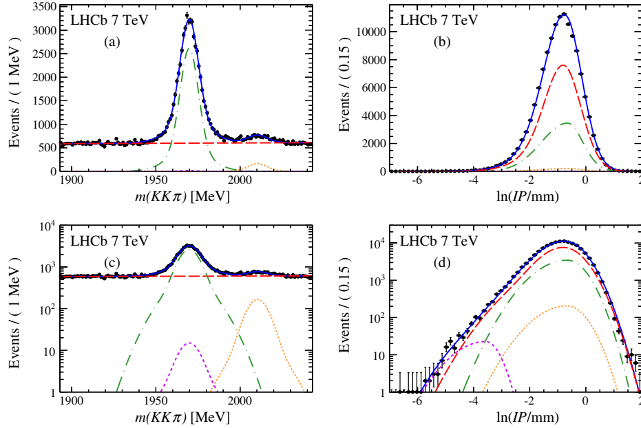
FIG. 1. Fits to the K^+K^-\pi^+ invariant mass (a) and \ln(IP/mm) (b) distributions for data taken at 7 TeV data integrated over 2 < \eta < 5 . The data are shown as solid circles (black), and the overall fits as solid lines (blue). The dot-dashed (green) curve shows the D_s^+ signal from b decay, while the dashed (purple) curve D_s^+ from prompt production. The dotted curve (orange) shows the D^{*+} component. The dashed line (red) shows the combinatorial background. The same fits using a logarithmic scale are shown in (c) and (d).
