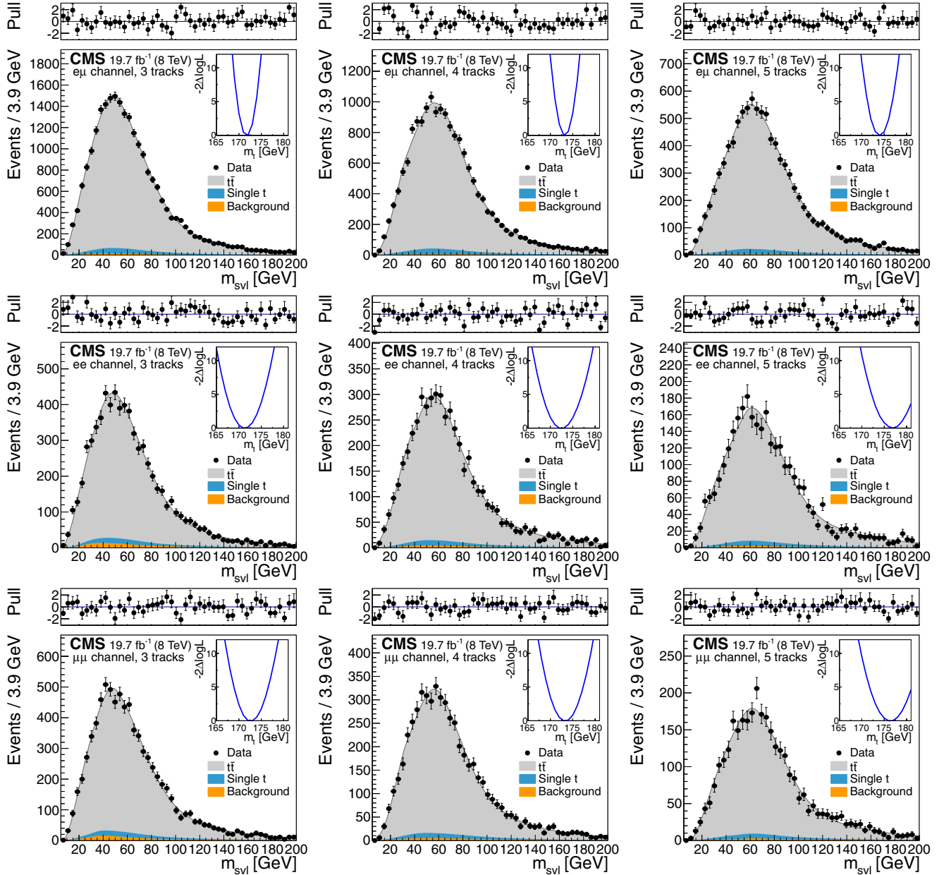
FIG. 6. Template fits to the observed m_{\text{svl}} distributions for the three dilepton channels ( e\mu , ee , \mu\mu from top to bottom row), and for exactly three, four, and five tracks assigned to the secondary vertex (from left to right column). The top panels show the bin-by-bin difference between the observed data and the fit result, divided by the statistical uncertainty (pull). The inset shows the scan of the negative log-likelihood as a function of the calibrated top quark mass, accounting only for the statistical uncertainty, when performed exclusively in each event category.
