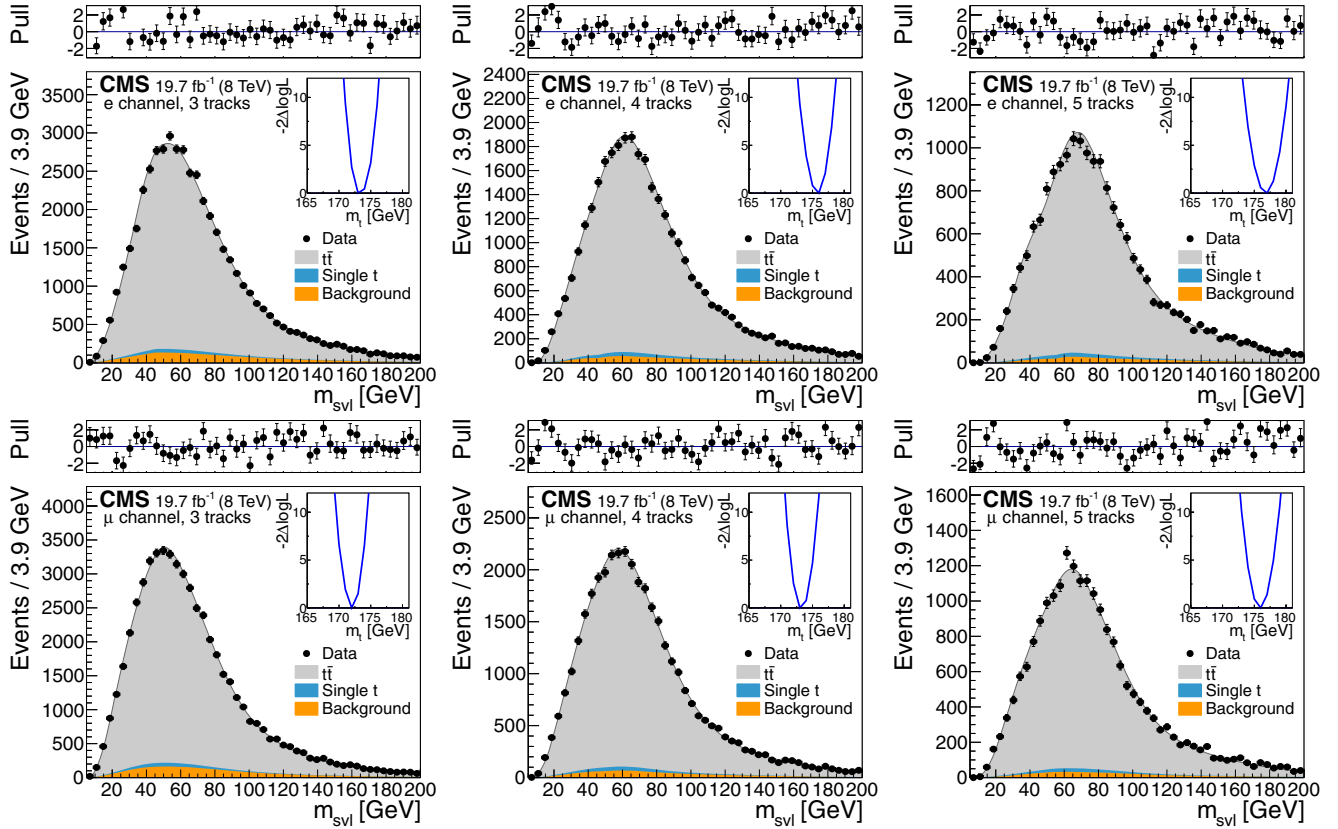
FIG. 7. Template fits to the observed m_{\text{svl}} distributions for the semileptonic channels ( e and \mu from top to bottom row), and for exactly three, four, and five tracks assigned to the secondary vertex (from left to right column). The top panels show the bin-by-bin difference between the observed data and the fit result, divided by the statistical uncertainty (pull). The inset shows the scan of the negative log-likelihood as a function of the calibrated top quark mass, accounting only for the statistical uncertainty, when performed exclusively in each event category.
