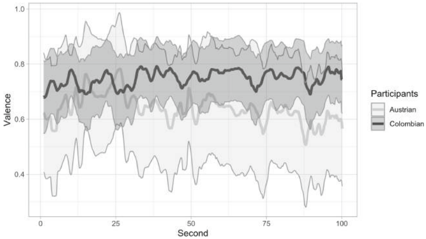
Fig. 2. Valence score means and 95%-CIs.
