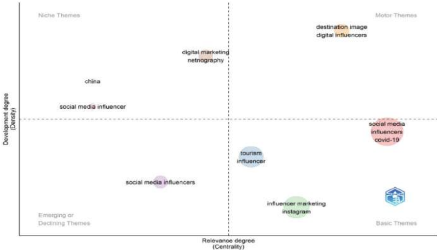
Fig. 6. Thematic map.
