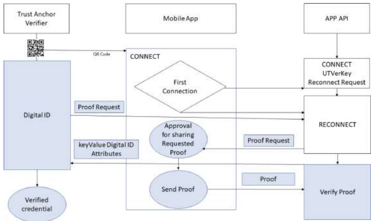
Fig. 3. Self-Identification architecture using cryptographic signatures
