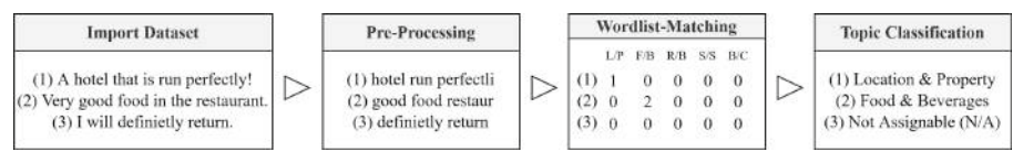
Fig. 1. Lexicon-based topic detection
