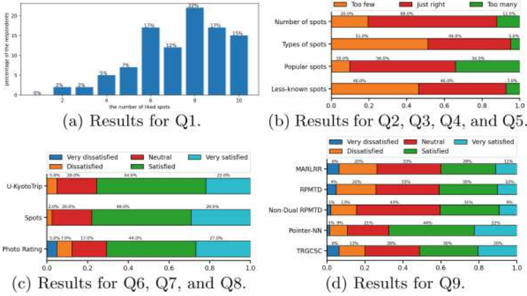
Fig. 3. Survey results.
