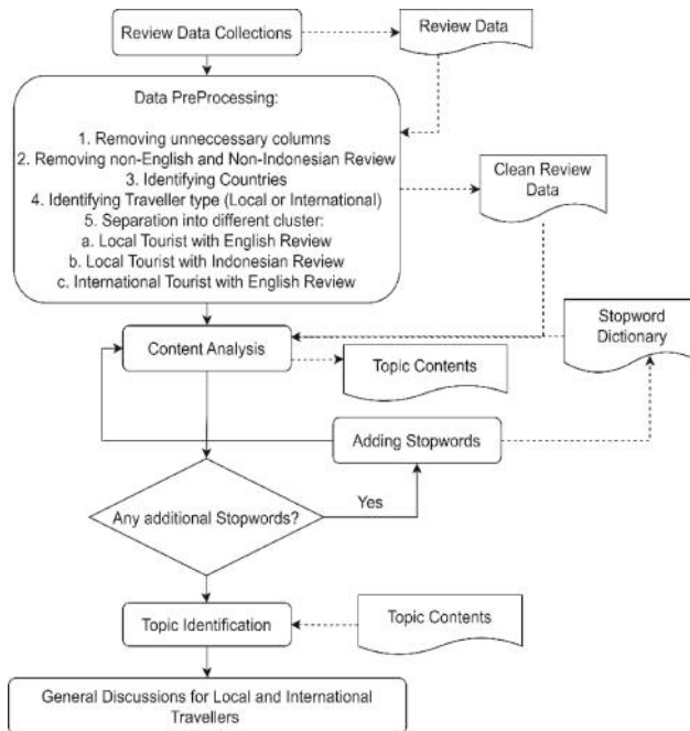
Fig. 1. Research Methodology
