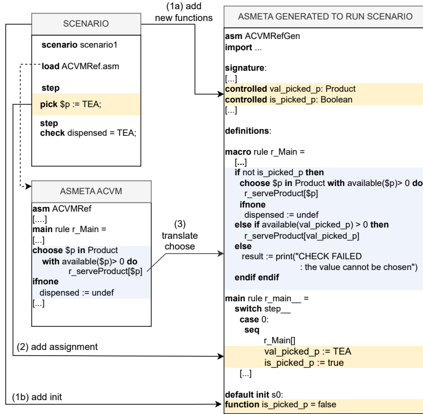
Fig. 2: Translation of pick in Asmeta for scenario1 of ACVMRef specification
