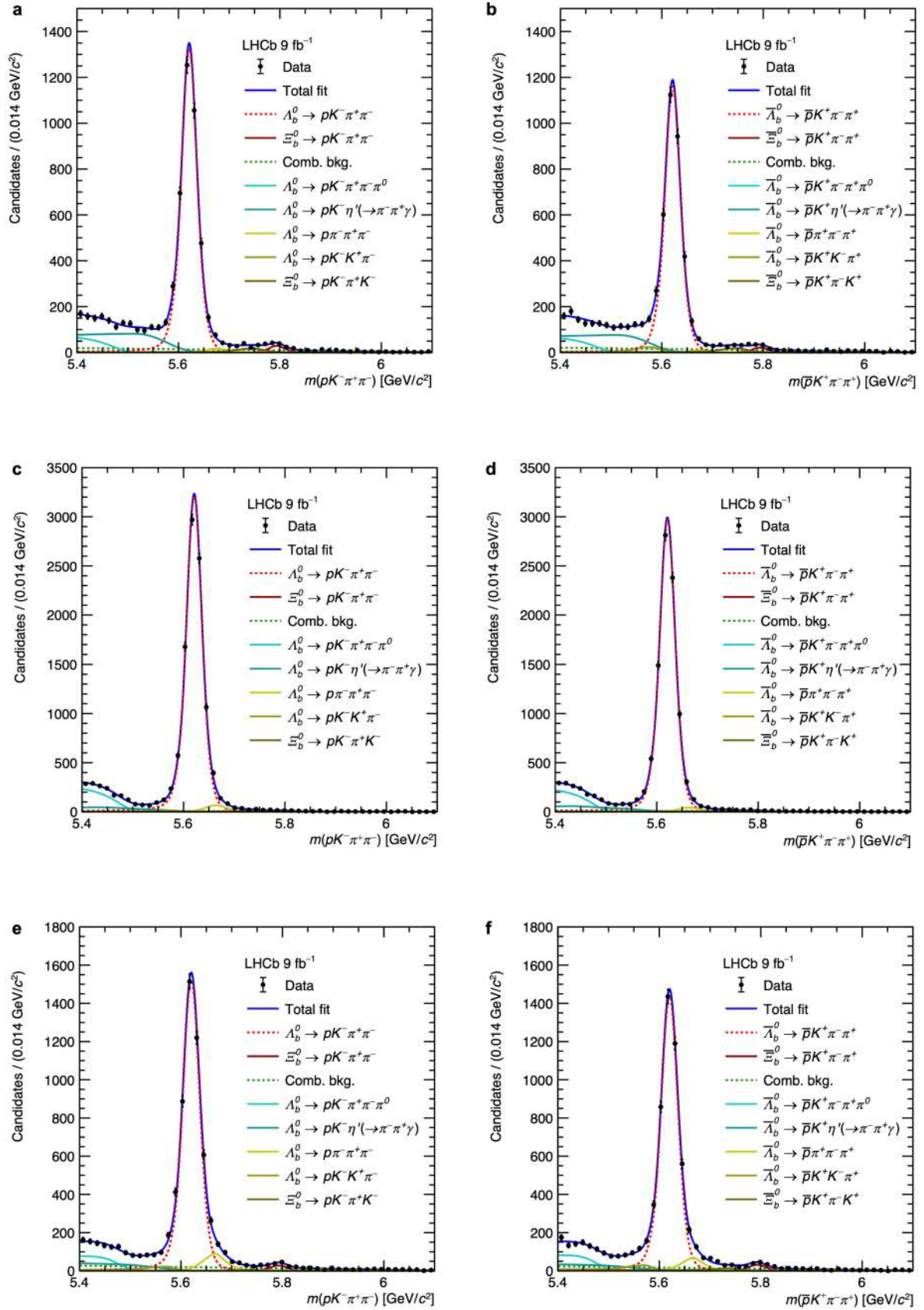
Extended Data Fig. 3 | Mass distributions in regions of phase space with the fit projections also shown. Mass distributions of \Lambda_b^0 \rightarrow p K^- \pi^+ \pi^- and \bar{\Lambda}_b^0 \rightarrow \bar{p} K^+ \pi^- \pi^+ for (a, b) \Lambda_b^0 \rightarrow R(p K^-) R(\pi^+ \pi^-) , (c, d) \Lambda_b^0 \rightarrow R(p \pi^-) R(\pi^+ K^-) , and (e, f) \Lambda_b^0 \rightarrow R(K^- \pi^+ \pi^-) p decays.
