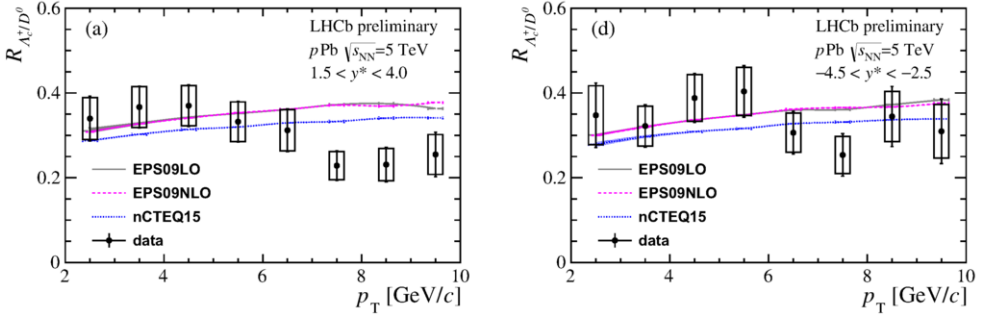
Fig. 4. The prompt \Lambda_C over D_0 production ratio at forward and at backward rapidity in p\text{Pb} collisions at \sqrt{s_{NN}} = 5 TeV measured by LHCb [12].
