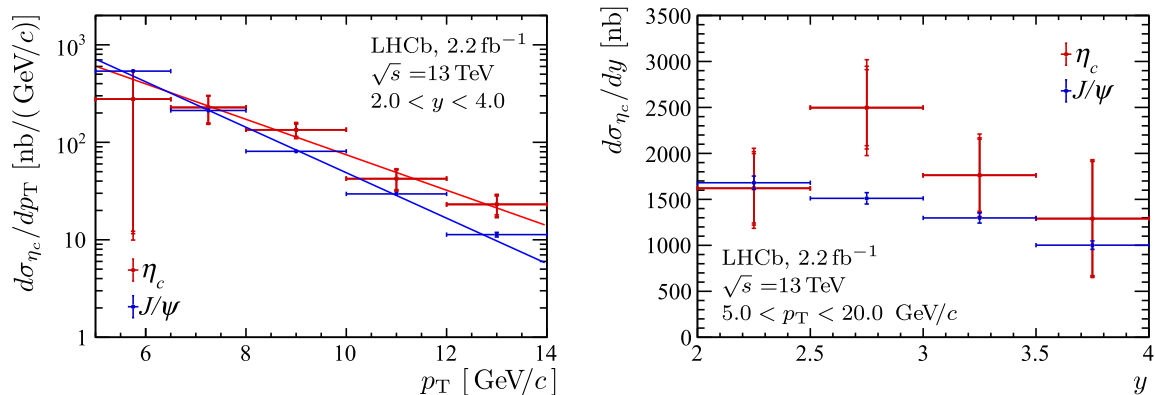
Fig. 6 Measurement of the differential prompt production cross-section of the (red) \eta_c and (blue) J/\psi mesons [15] in bins of (left) p_T and (right) y . The error bars show following uncertainties for \eta_c produc-
