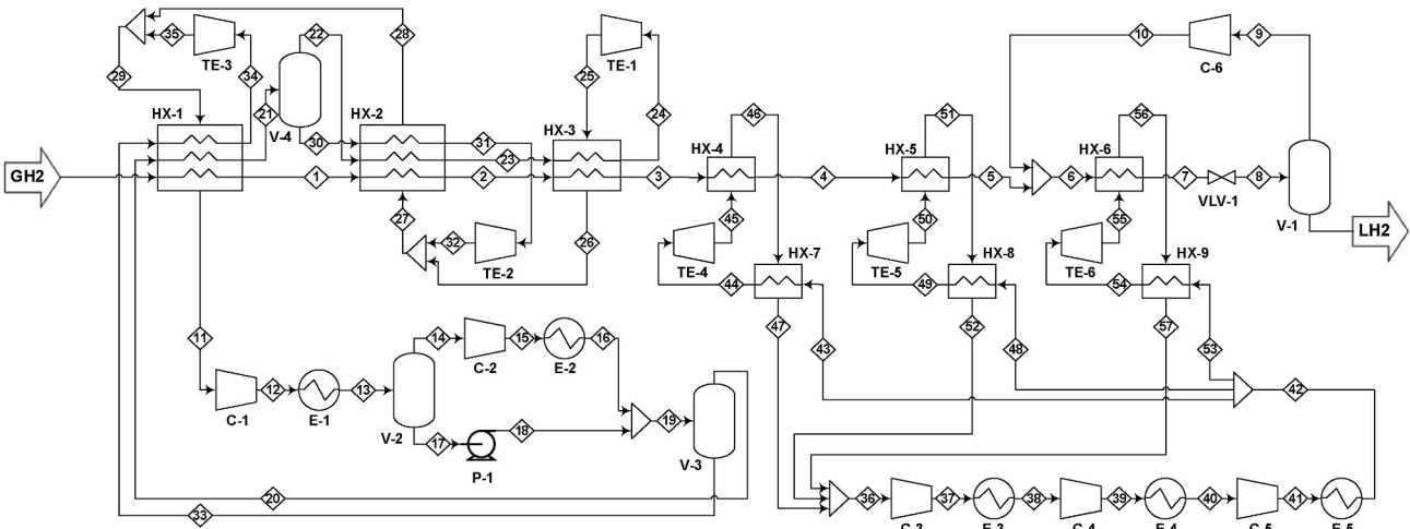
Fig. 4. Process scheme of MR cascade process for hydrogen liquefaction.
