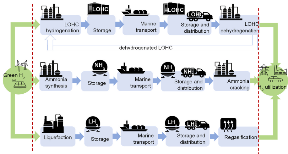
Fig. 1. H 2 value chain for the different carriers analysed.
